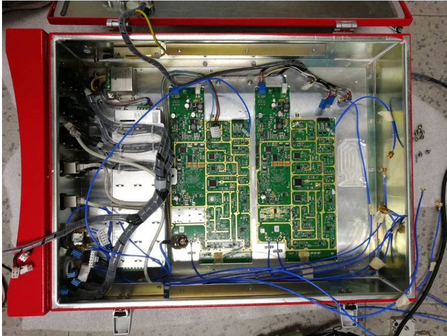
EUT – Cover off View 5 (Model: RH-7W22B-D)
