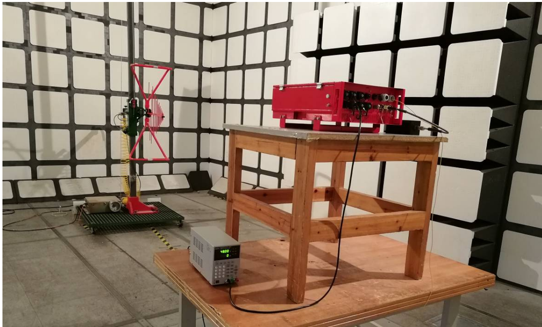
Transmitting Radiated Emissions Tested - Rear View (Below 1 GHz)
