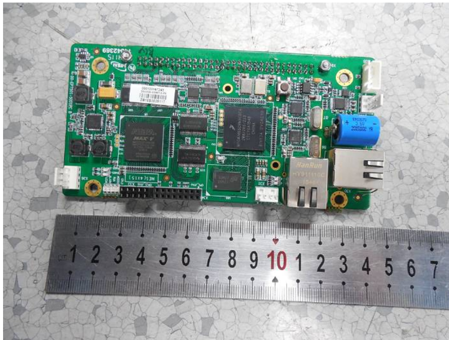
EUT – MCU Board Top View
