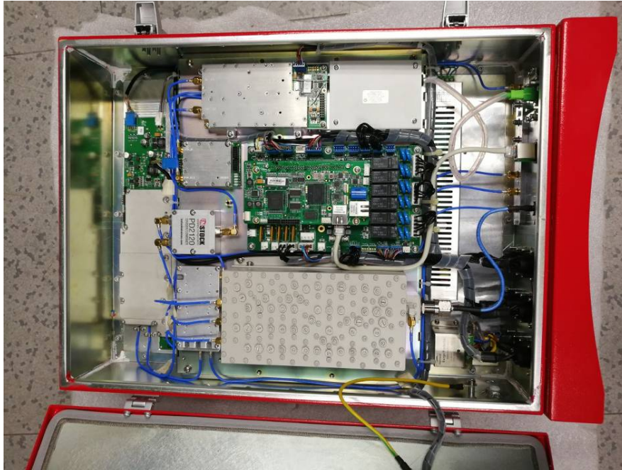
EUT – Cover off View 1 (Model: RH-7W22B-R)
