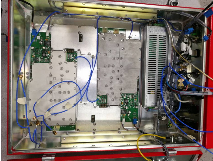
EUT – Cover off View 3 (Model: RH-7W22B-R)
