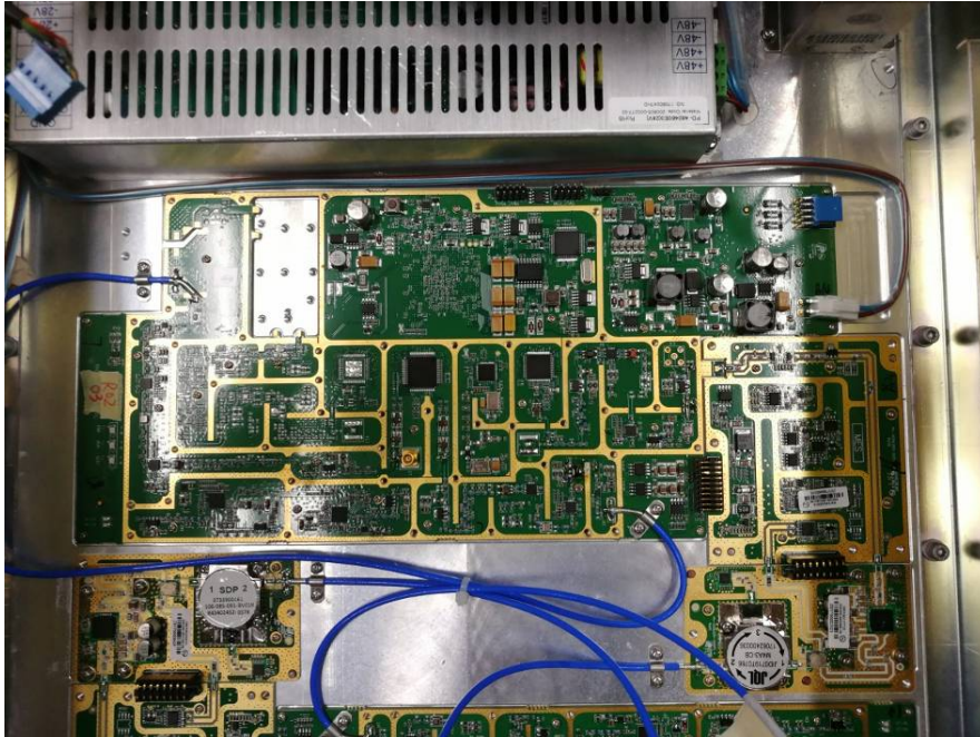
EUT – Integrated Module View
