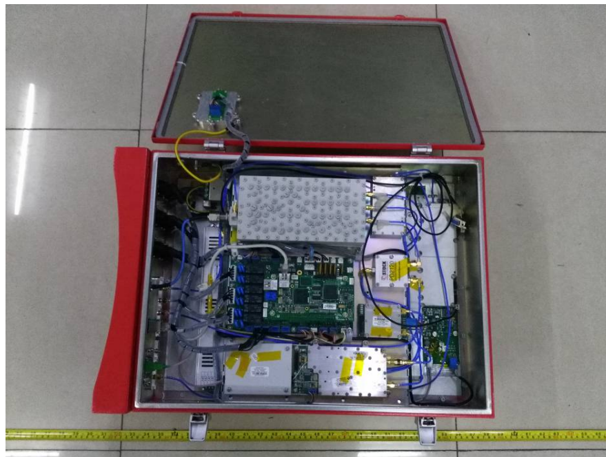
EUT – Cover off View 4 (Model: RH-7W22B-R-AC)
