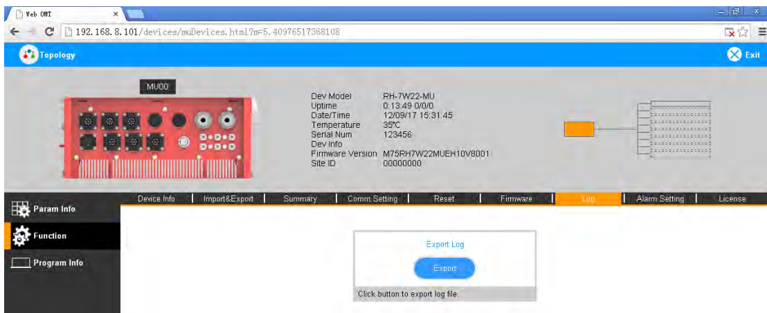
Figure 36: Function – Log
