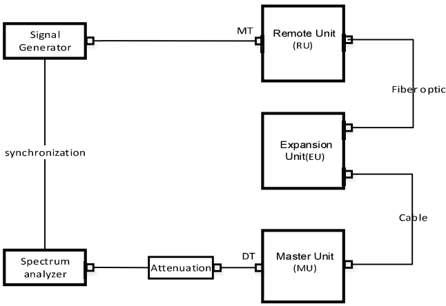
Figure 11.6-2 Uplink connection diagram
