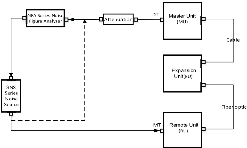
Figure 11.7-2 Uplink connection diagram
