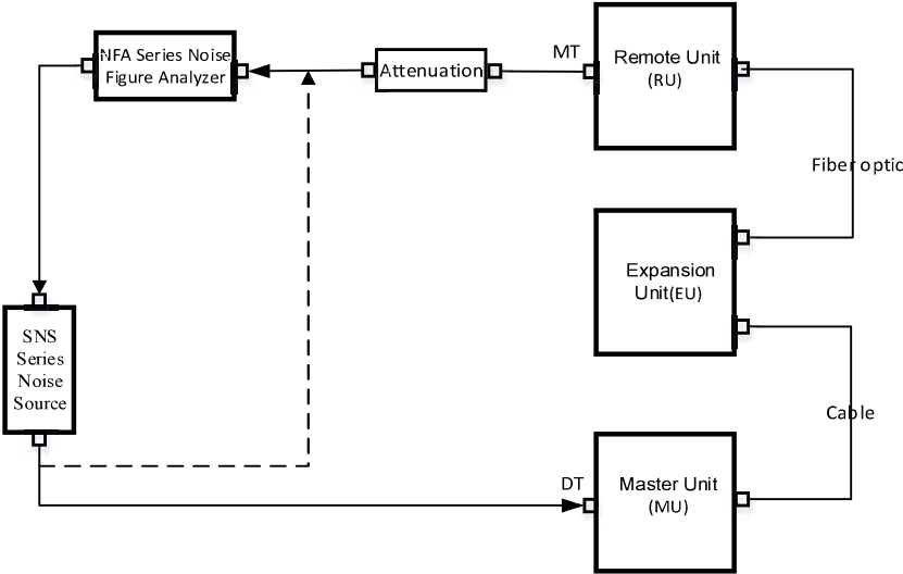
Figure 11.7-1 Downlink connection diagram
