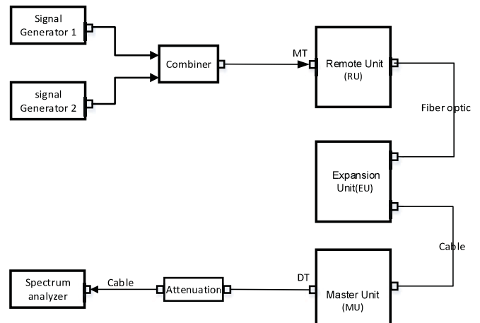
Figure 11.8-2 Uplink connection diagram
