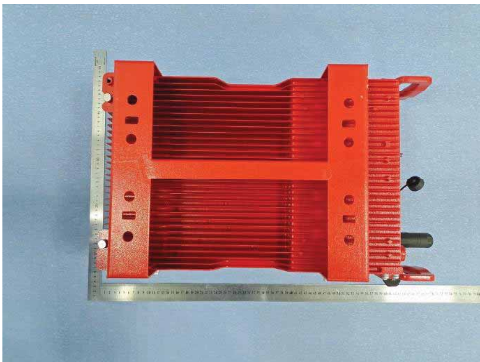
Bottom surface
