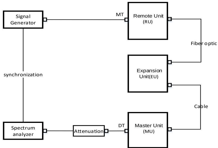
Figure 11.9-2 Uplink connection diagram
