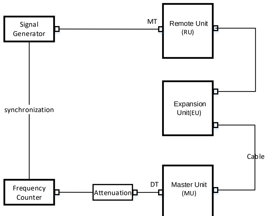
Figure 11.10-2 Uplink connection diagram
