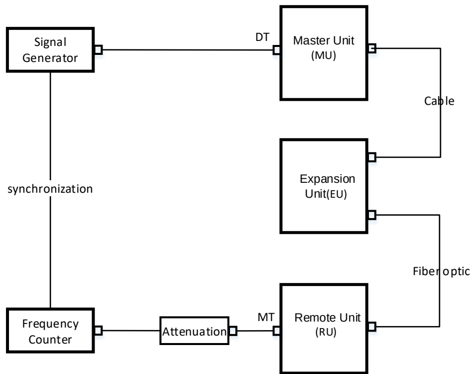
Figure 11.10-1 Downlink connection diagram
