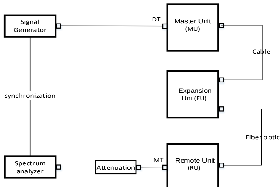
Figure 11.9-1 Downlink connection diagram
