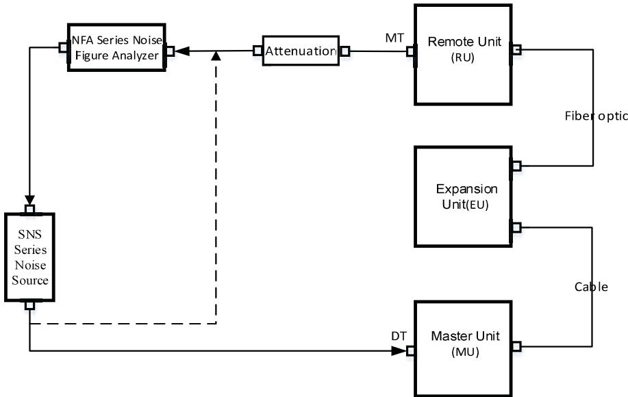
Figure 11.7-1 Downlink connection diagram
