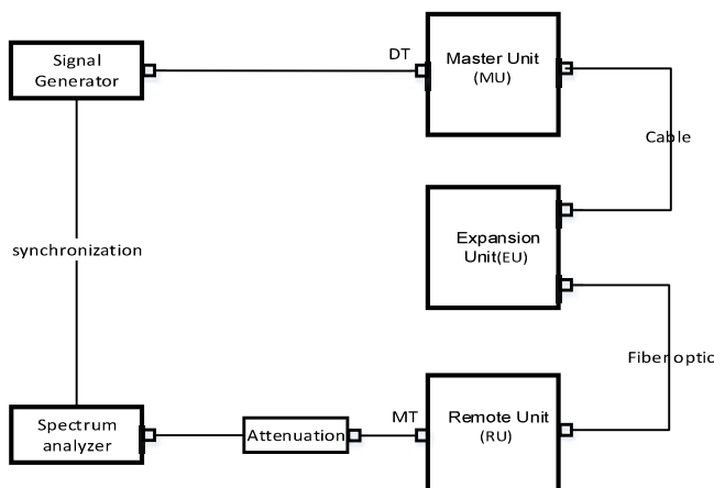
Figure 11.3-1 Downlink connection diagram
