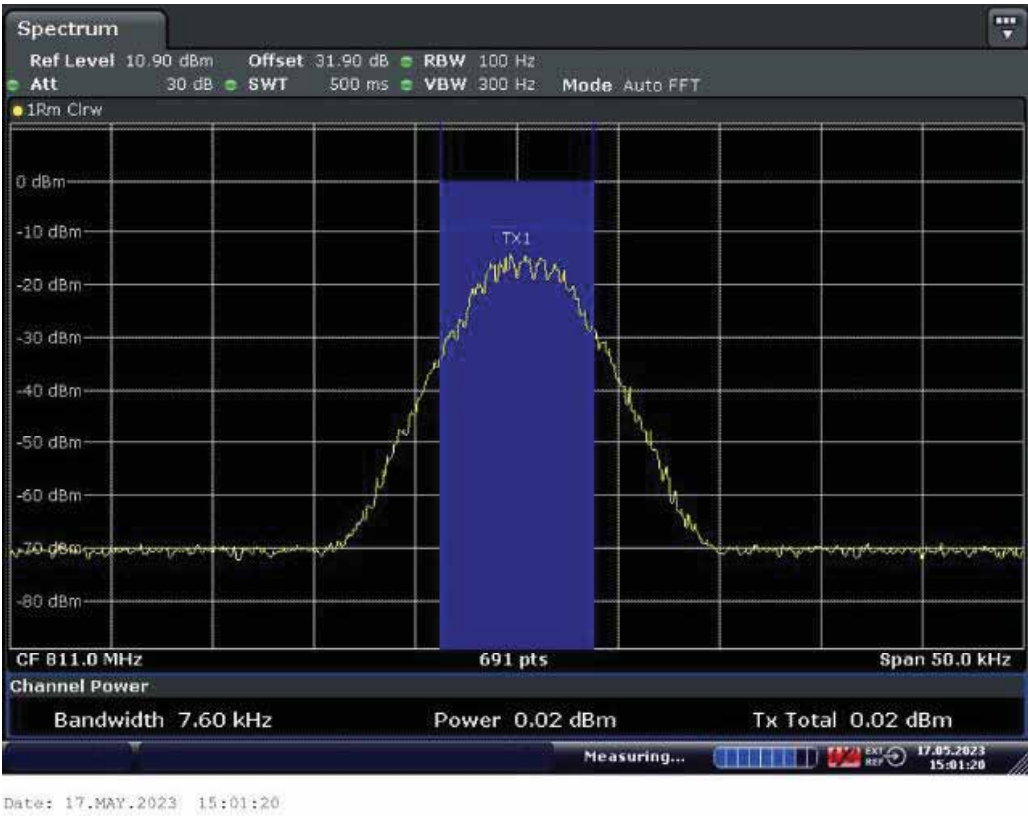
Middle Frequency: 811.0MHz MHz, Input occupied BW
