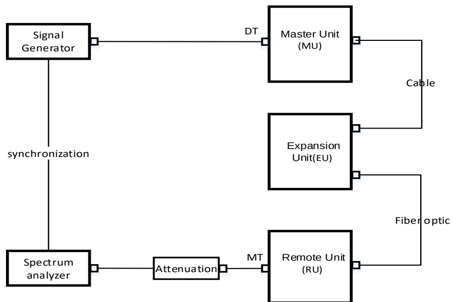
Figure 11.5-1 Downlink connection diagram
