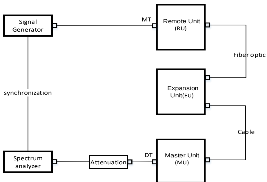
Figure 11.5-2 Uplink connection diagram
