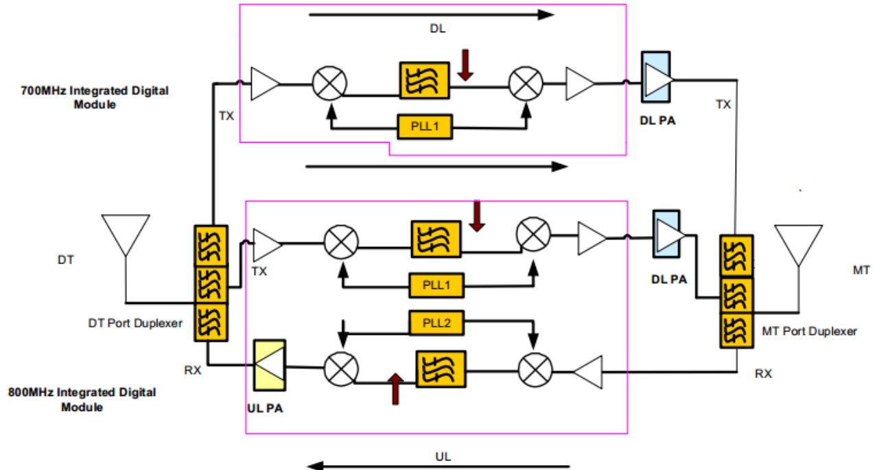
Figure 1: PS BDA Functional Block Diagram
