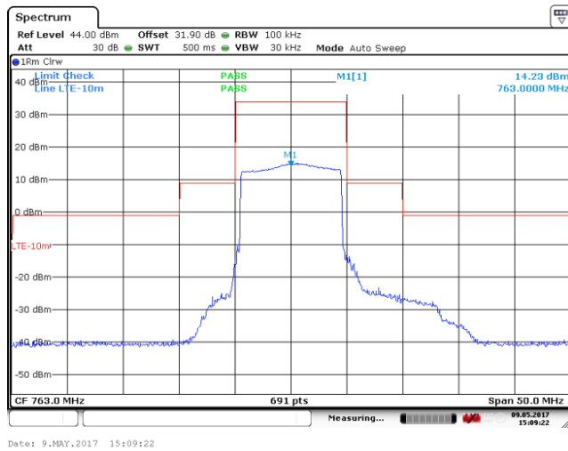
Downlink: 763.0MHz
