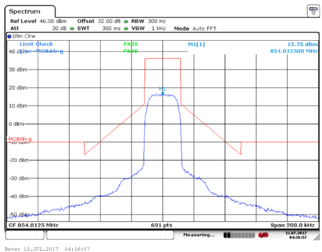
Low Frequency: 854.0125MHz (Mask G)
