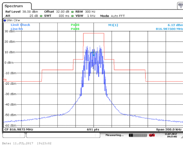
High Frequency: 816.9875MHz (Mask B)
