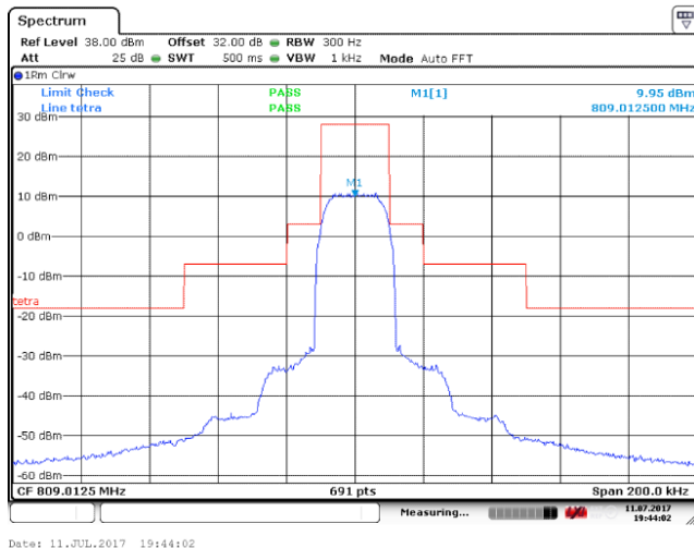
Low Frequency: 809.0125MHz (Mask B)
