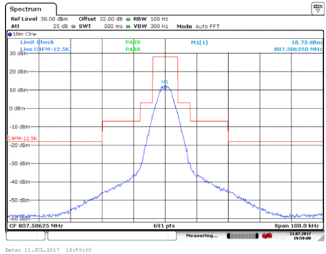
Mid Frequency: 807.50625MHz(Mask B)
