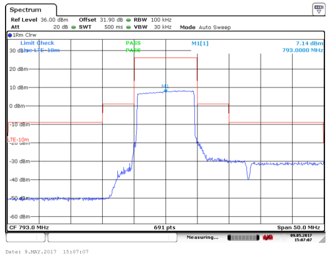
Uplink: 793.0MHz
