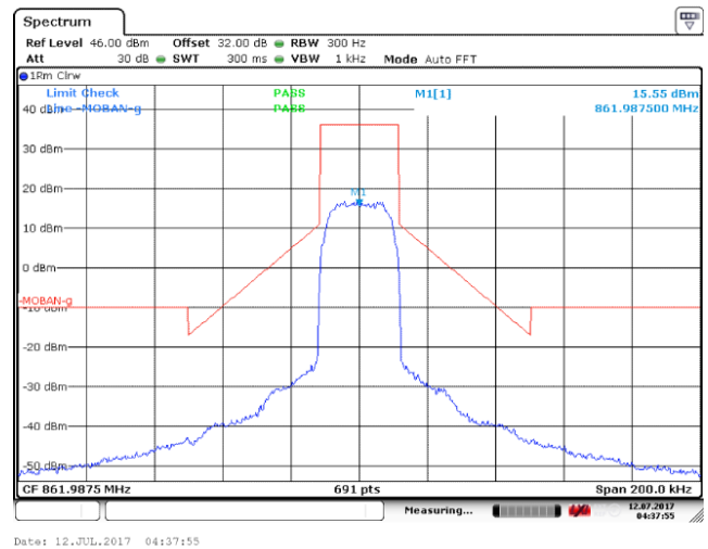
High Frequency: 861.9875MHz (Mask G)
