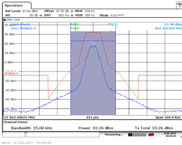
Mid Frequency: 852.50625MHz (Mask H)
