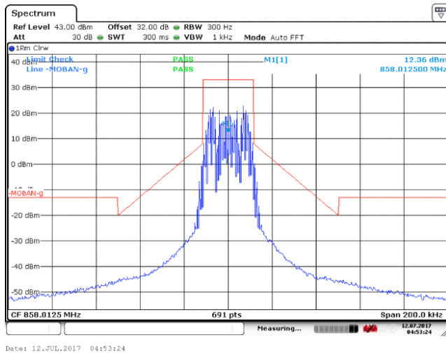
Mid Frequency: 858.0125MHz (Mask G)
