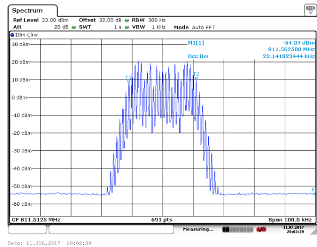
Mid Frequency: 811.5125MHz, Input occupied BW
