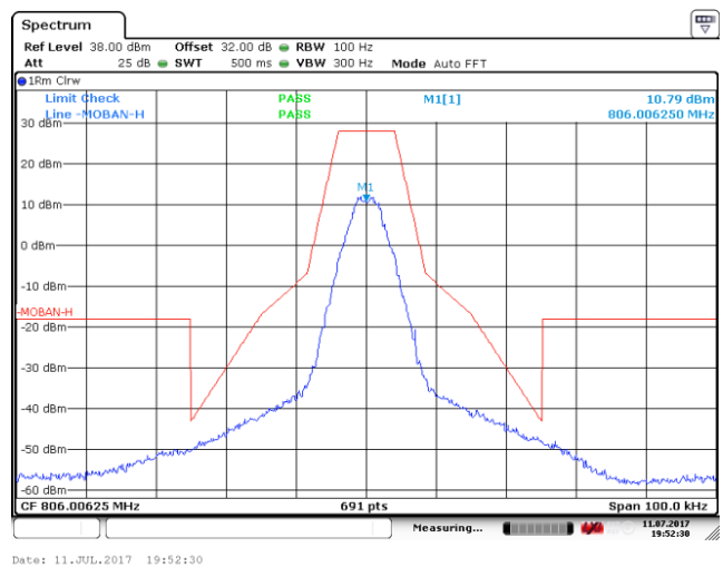
Low Frequency: 806.00625MHz (Mask H)
