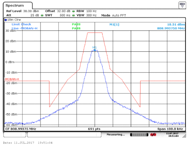
High Frequency: 808.99375MHz (Mask H)
