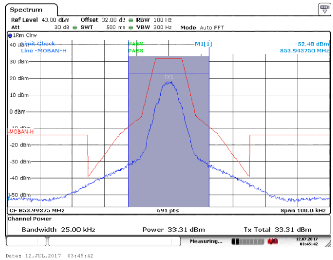
High Frequency: 853.99375MHz (Mask H)
