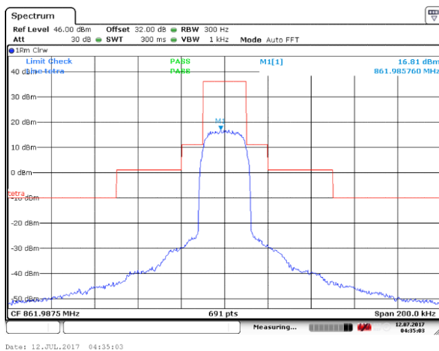
High Frequency: 861.9875MHz (Mask B)
