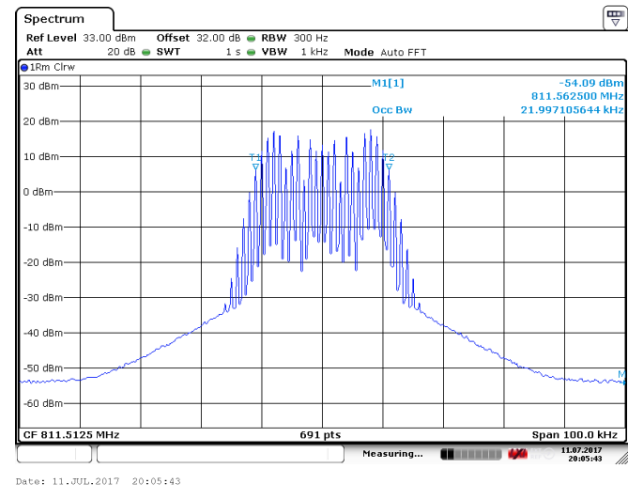
Mid Frequency: 811.5125MHz, Output occupied BW(with the input signal amplitude set 3 dB above the ALC threshold)
