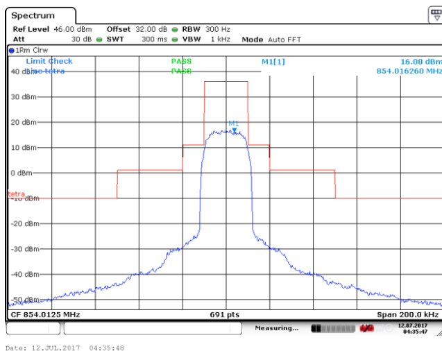
Low Frequency: 854.0125MHz (Mask B)
