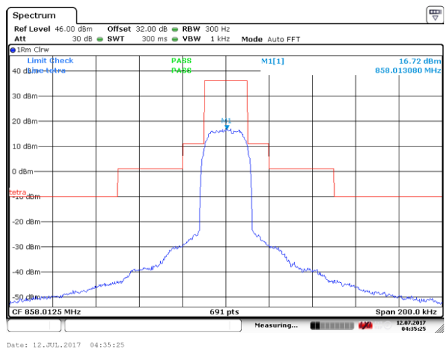
Mid Frequency: 858.0125MHz (Mask B)
