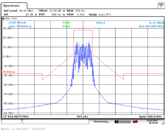
High Frequency: 816.9875MHz (Mask G)
