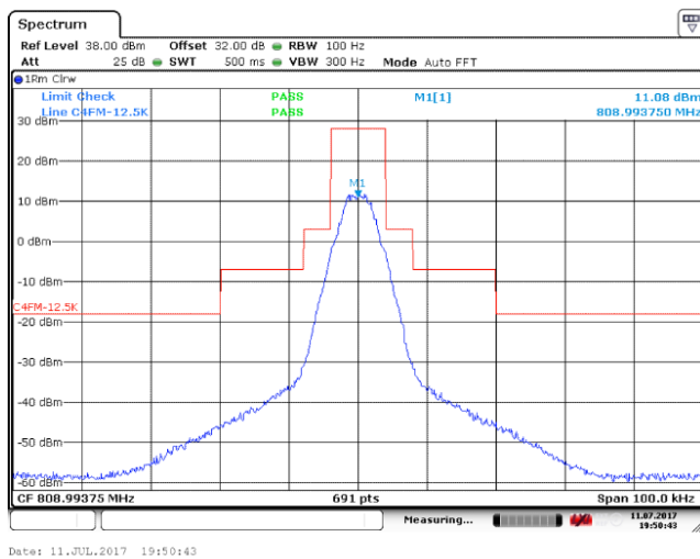
High Frequency: 808.99375MHz(Mask B)
