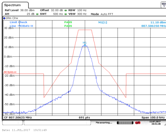
Mid Frequency: 807.50625MHz (Mask H)
