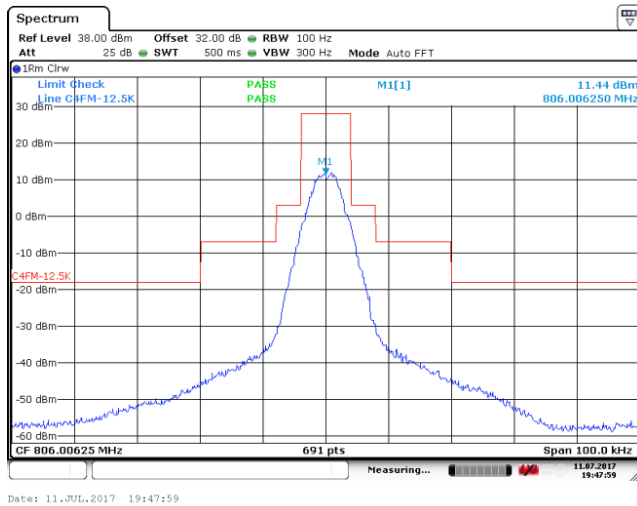
Low Frequency: 806.00625MHz(Mask B)
