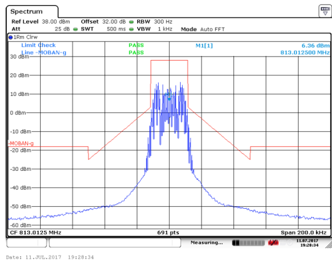
Mid Frequency: 813.0125MHz (Mask G)
