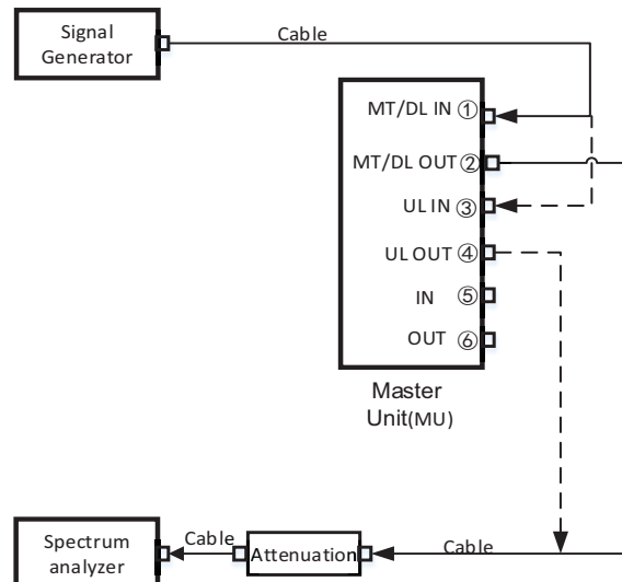
Figure 10.4-1 MU single device test connection diagram
