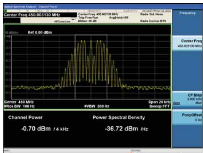
Input signal Low Frequency: 450.00313MHz
