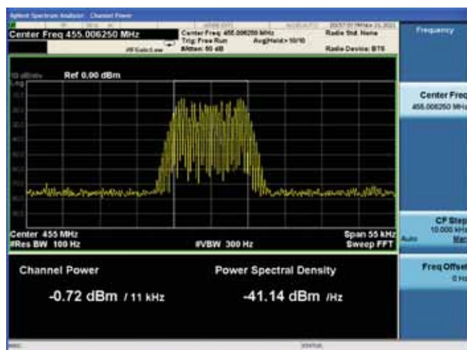
Input signal Low Frequency: 455.00625MHz
