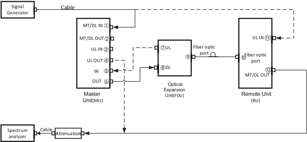
Figure 10.9-2 MU, FOU and RU system test connection diagram
