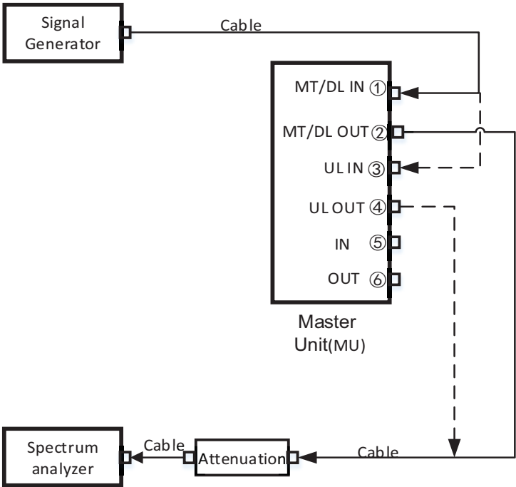
Figure 10.9-1 MU single device test connection diagram
