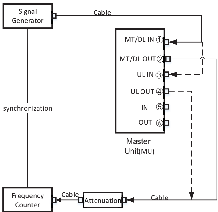
Figure 10.10-1 MU single device test connection diagram
