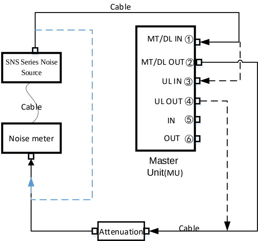
Figure 10.7-1 MU Single device test connection diagram
