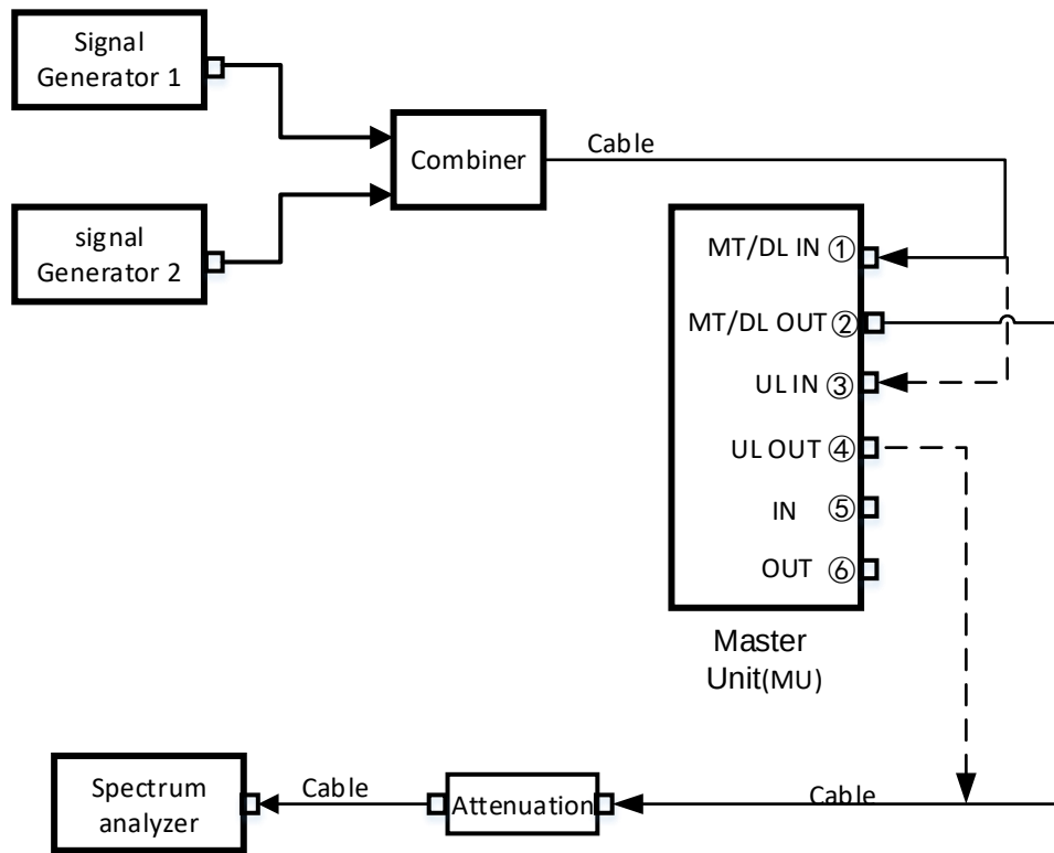
Figure 10.8-1 MU single device test connection diagram
