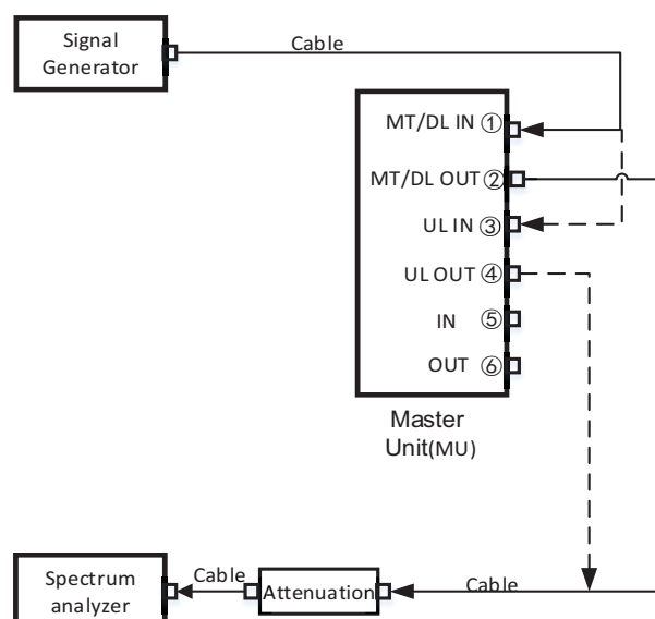
Figure 10.6-1 MU single device test connection diagram
