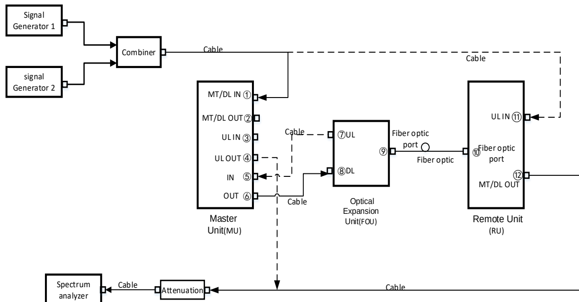
Figure 10.8-2 MU, FOU and RU system test connection diagram
