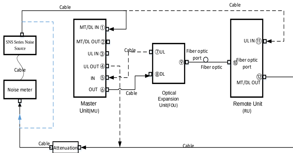
Figure 10.7-2MU, FOU and RU system test diagram
