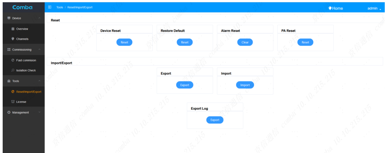
Figure 18: Reset/Import/Export Screen
