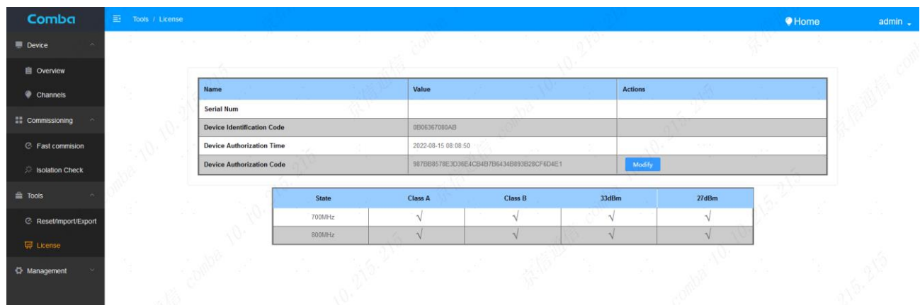
Figure 19: License Screen
