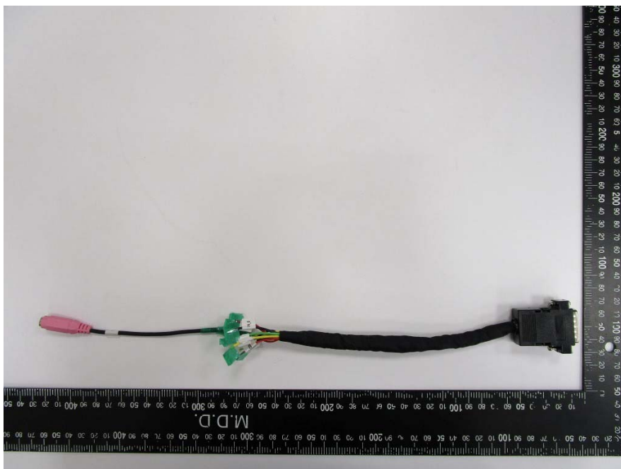
15 pin VGA to Audio cable
