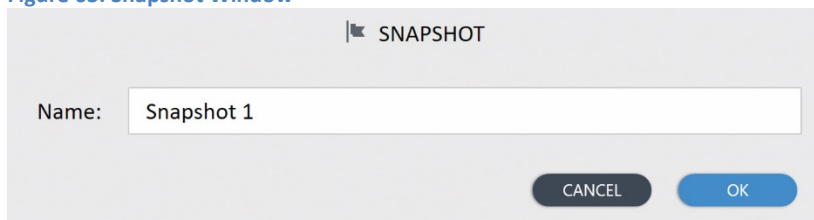
Figure 63. Snapshot Window
