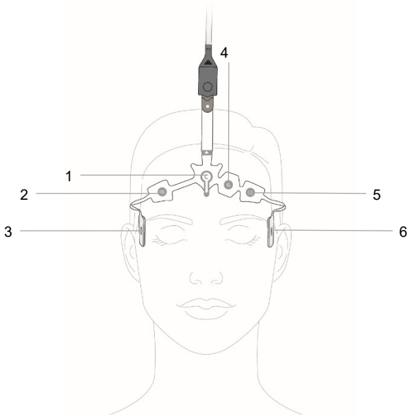
Figure 26. Sensor Positioning for Four-channel Sensor
