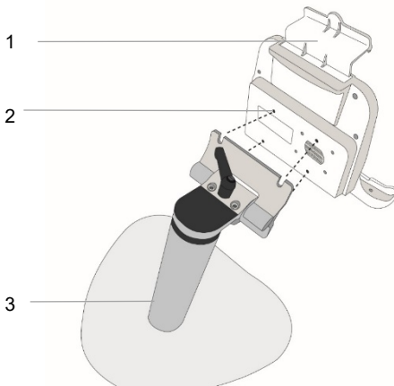
Figure 16. Setup with GCX Desktop Mount
