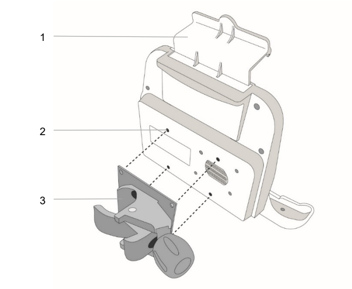
Figure 15. Setup with GCX Clamp Mount
