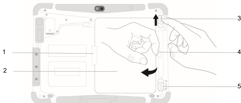
Figure 14. Battery Assembly/Disassembly
