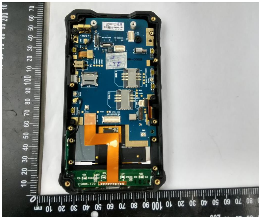
EUT UNCOVER VIEW 6
