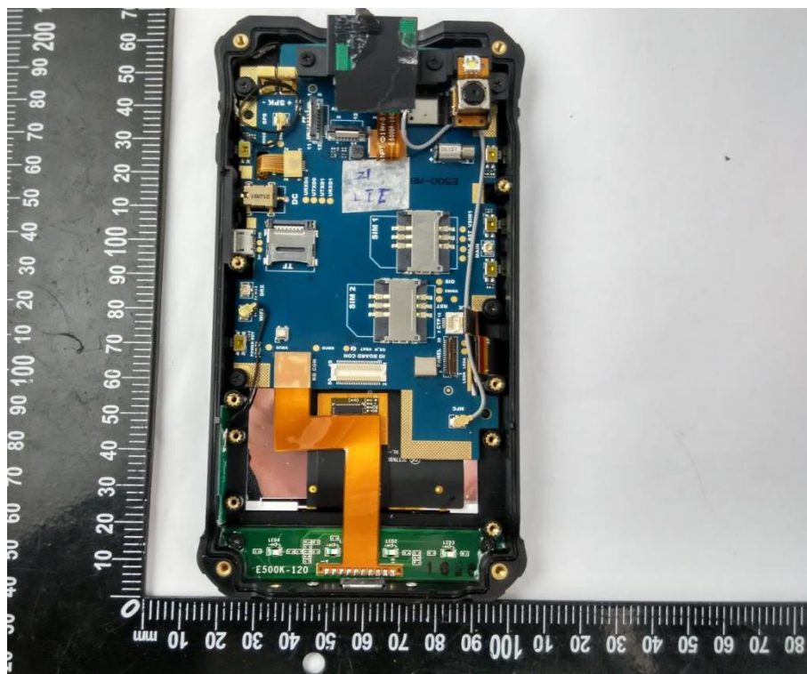
EUT UNCOVER VIEW 4
