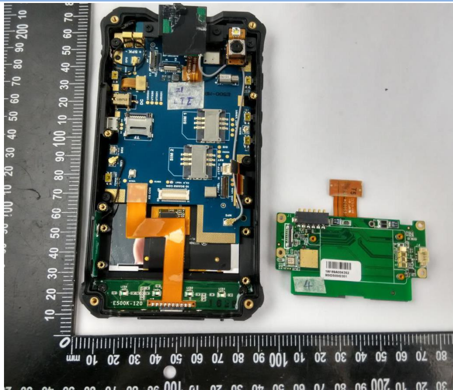
EUT UNCOVER VIEW 3
