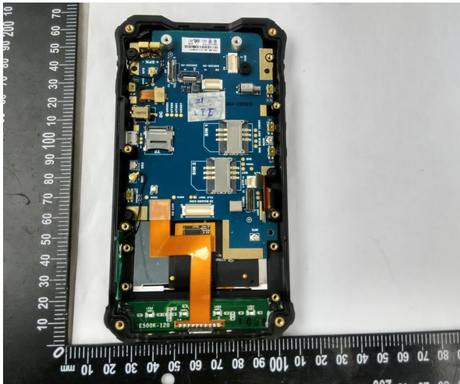
EUT UNCOVER VIEW 6
