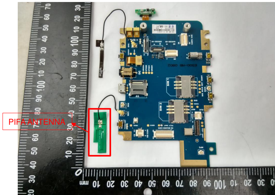
MAIN BOARD TOP VIEW 2
