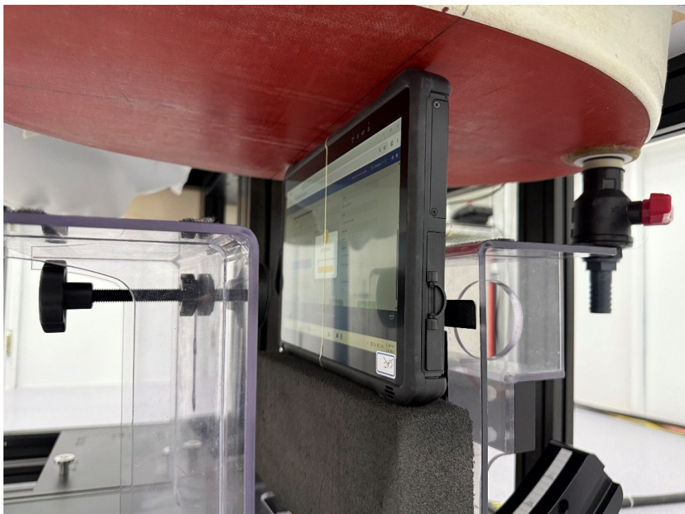
Description: Body Top Position with 0 mm gap
