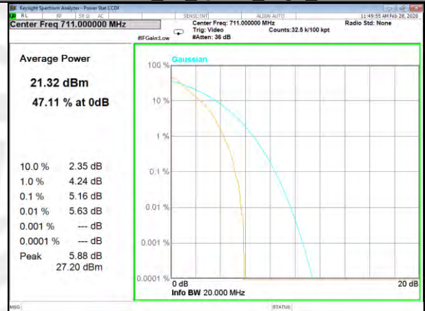
B12_50_Q16_High_
