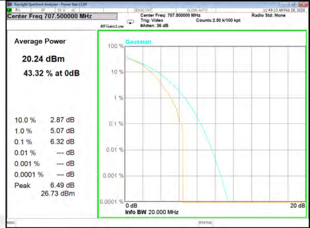
B12_50_QPSK_High_
