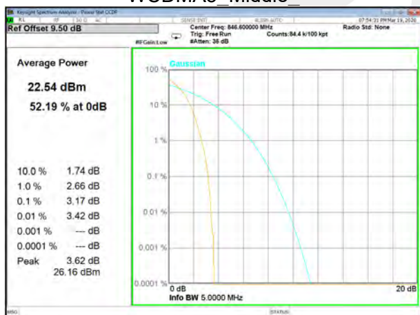
WCDMA5_Higher
