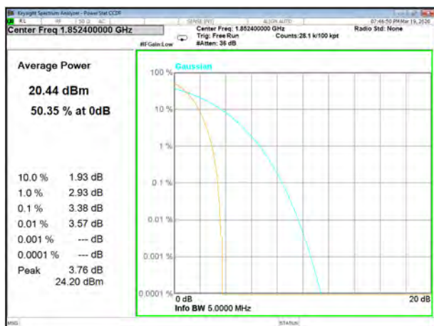
HSPA2_Lower_
