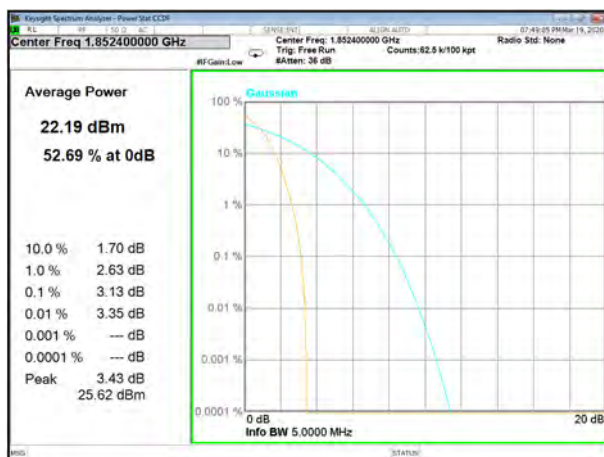
HSDPA2_Lower
