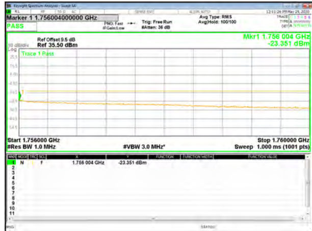
B4 HSDPA High Band edge
