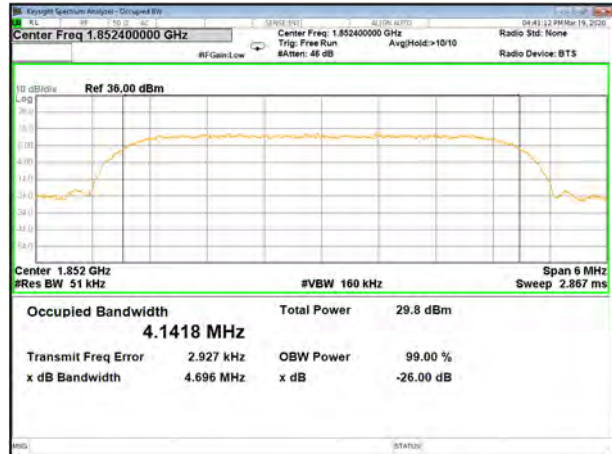
B2 HSDPA Lower 26BW and 99%
