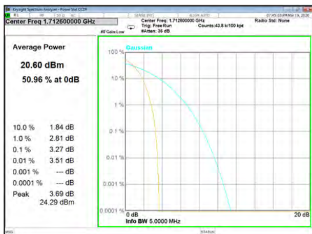
HSPA4_Lower_
