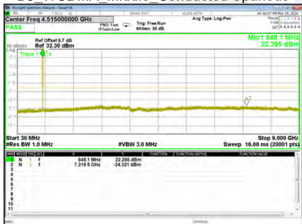
B5_WCDMA_Higher_Conducted_Spurious
