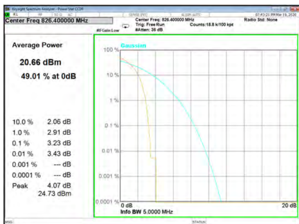
HSPA5_Lower_
