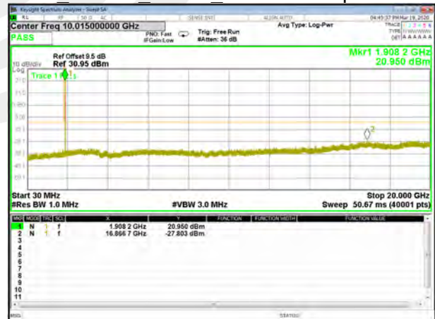
B2_HSDPA_Higher_Conducted Spurious
