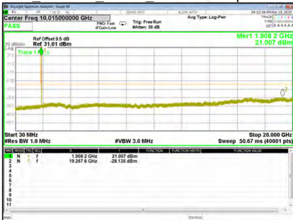
B2_WCDMA_Higher_Conducted Spurious
