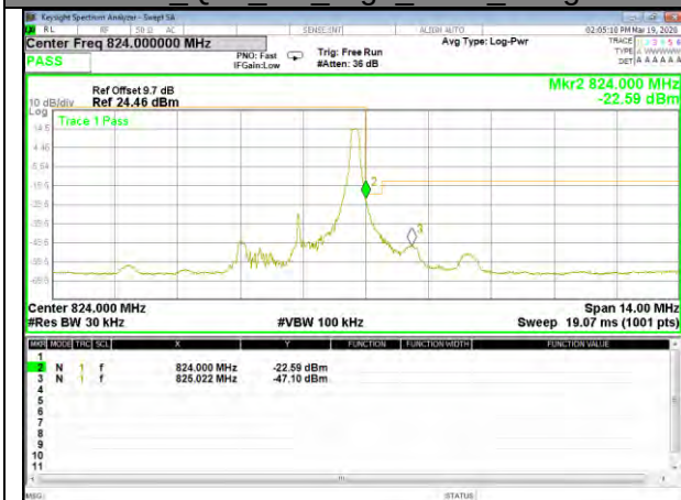
B26_QPSK_5M_Low_1-RB_Bedge
