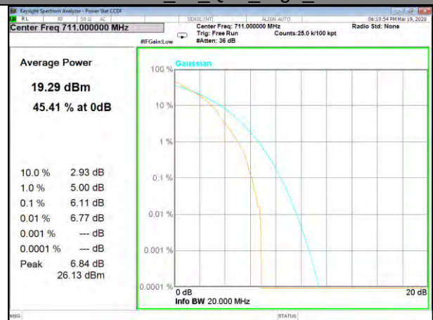
B12_50_Q16_High_
