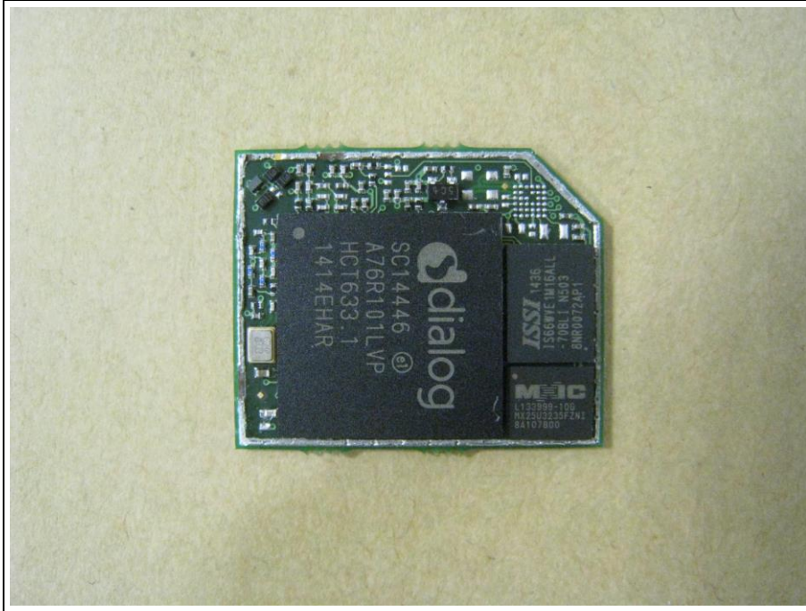
RADIO PART WITHOUT SHIELDING TOP
