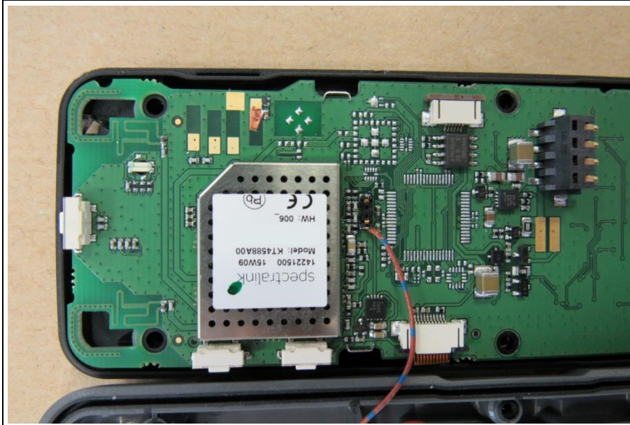
VARIANT 7622 PCB BOTTOM
