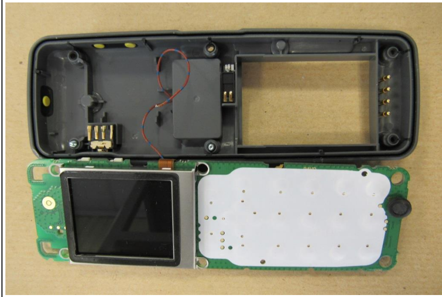
VARIANT 7622 PCB TOP
