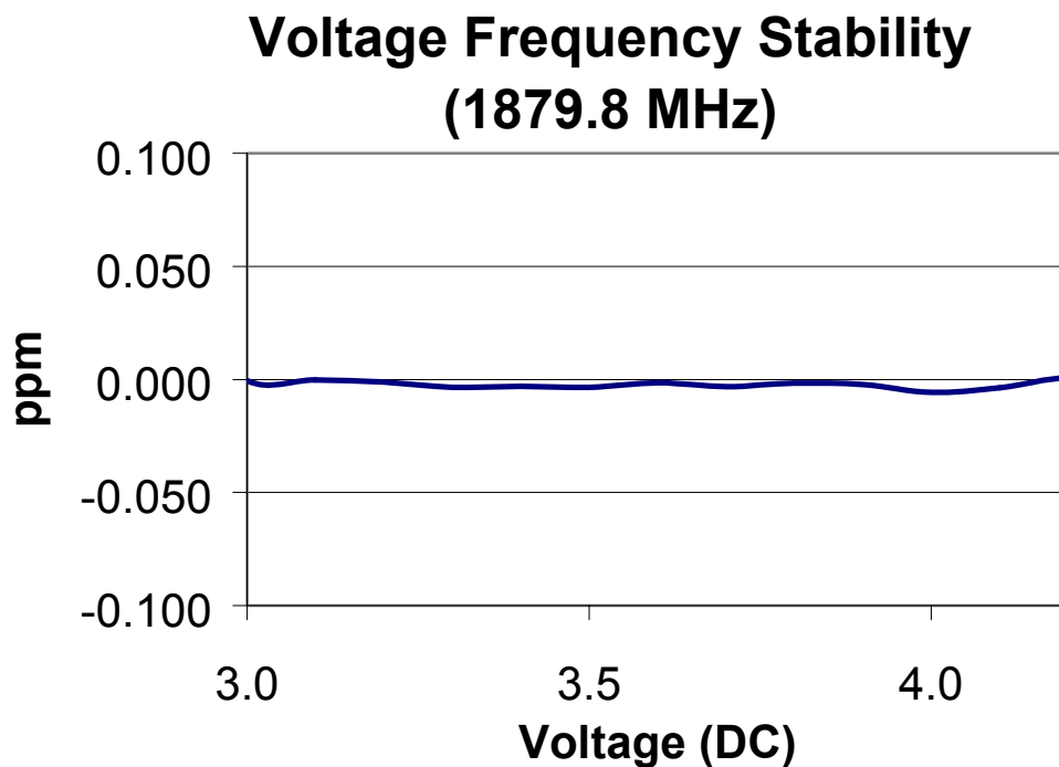
PLOT 9-4: VOLTAGE FREQUENCY STABILITY DATA - §2.1055 (1900 MHZ GSM BAND)
