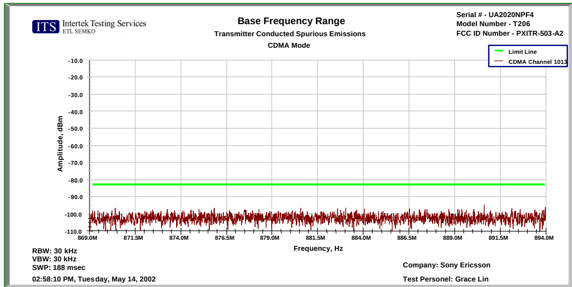
Figure 8.3-15: Emissions in base frequency range – CDMA 800 Channel 1013
