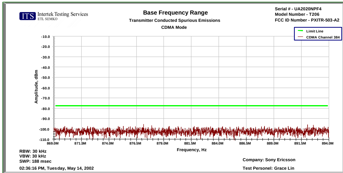
Figure 8.3-13: Emissions in base frequency range – CDMA 800 Channel 384
