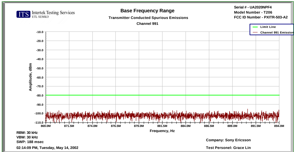
Figure 8.3-12: Emissions in base frequency range – AMPS Channel 991
