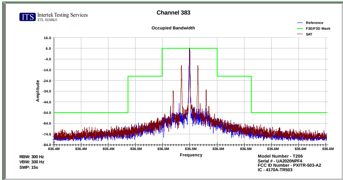
Figure 7.3-1: Occupied Bandwidth – SAT
