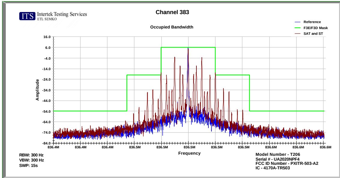
Figure 7.3-3: Occupied bandwidth – SAT and ST
