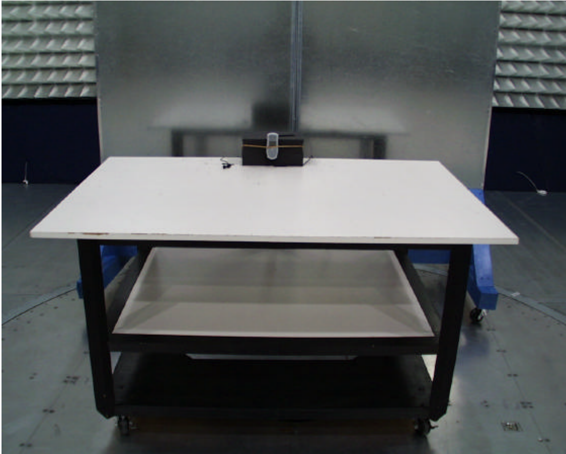
Figure 10.4-1: Configuration photograph, AC mains conducted emission, front view
