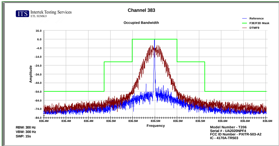
Figure 7.3-4: Occupied bandwidth – DTMF9
