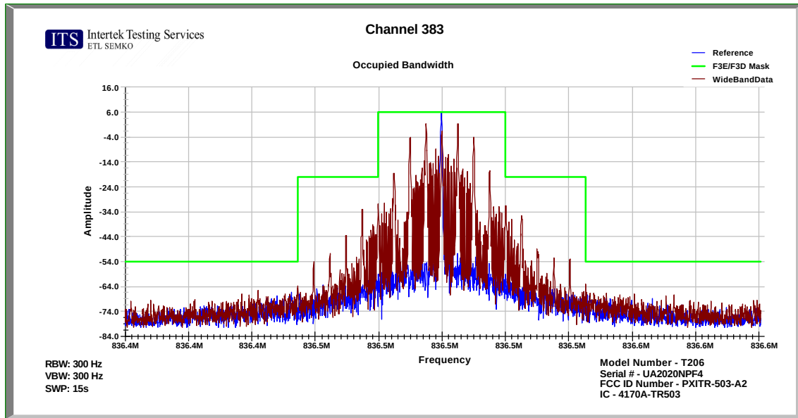
Figure 7.3-7: Occupied Bandwidth – 10kb Wideband Data
