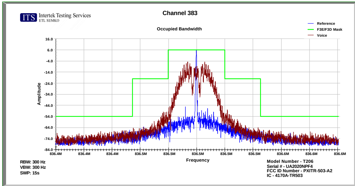
Figure 7.3-5: Occupied Bandwidth – Voice
