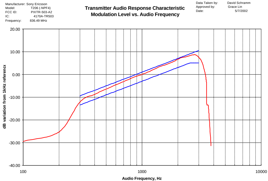
Figure 6.3-1: Audio Filter Characteristics
