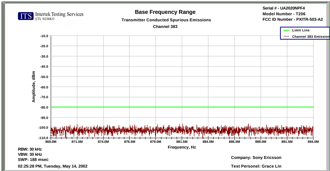
Figure 8.3-10: Emissions in base frequency range – AMPS Channel 383
