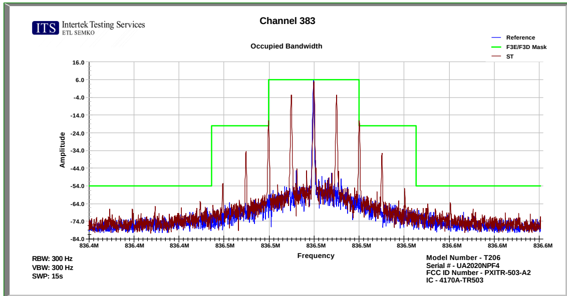
Figure 7.3-2: Occupied Bandwidth – Signaling Tone
