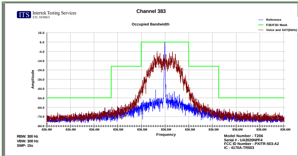
Figure 7.3-6: Occupied bandwidth – Voice and SAT
