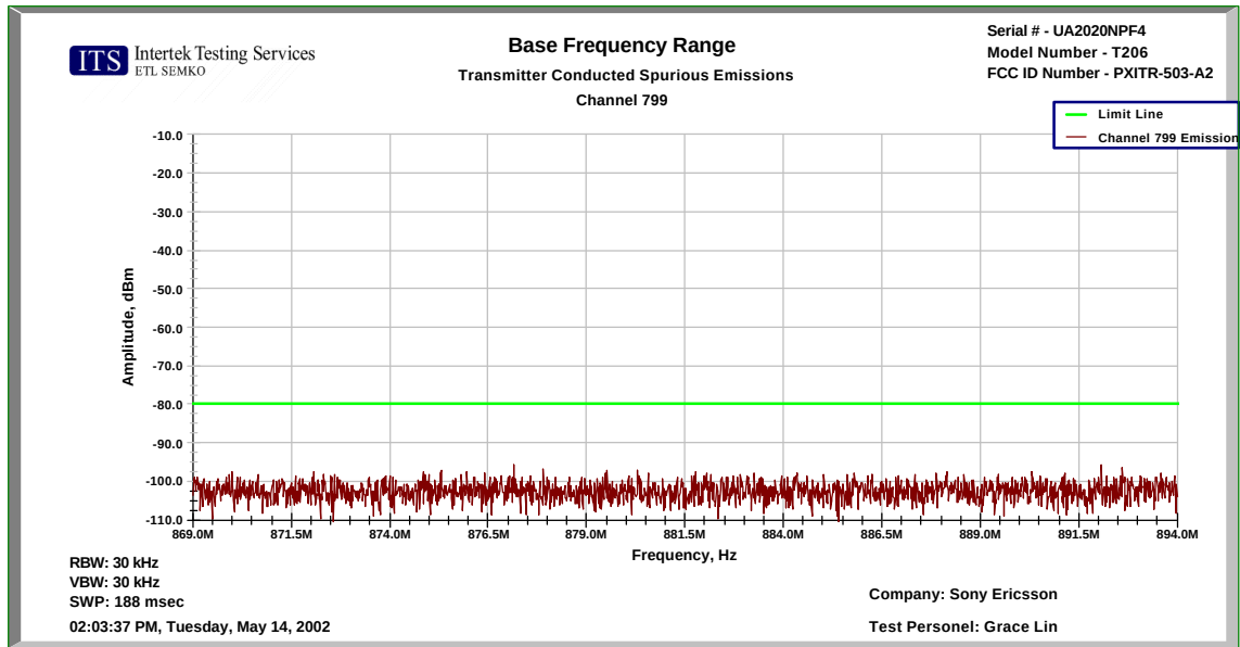
Figure 8.3-11: Emissions in base frequency range – AMPS Channel 799
