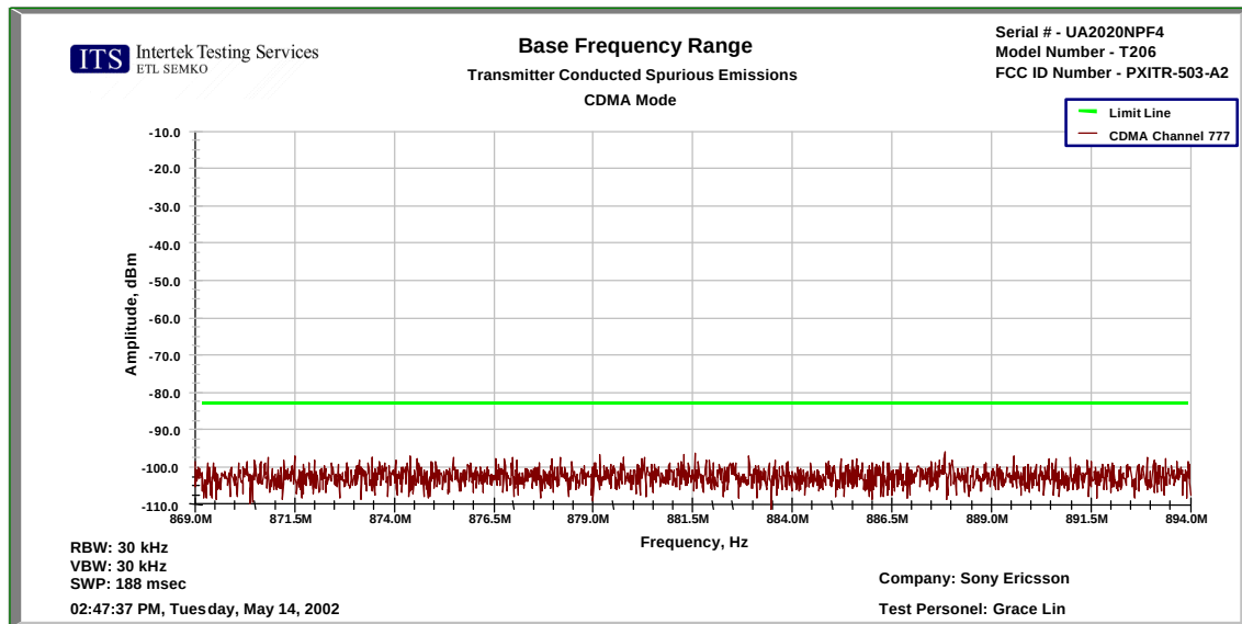
Figure 8.3-14: Emissions in base frequency range – CDMA 800 Channel 777
