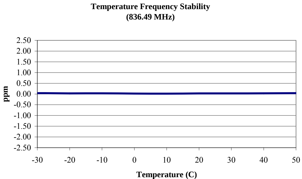
PLOT 9-1: TEMPERATURE FREQUENCY STABILITY DATA - §2.1055 (800 MHZ TDMA BAND)
