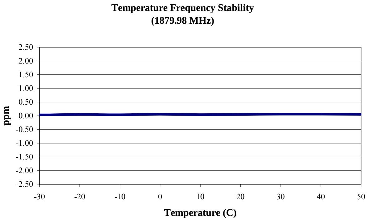
PLOT 9-2: TEMPERATURE FREQUENCY STABILITY DATA - §2.1055 (1900 MHZ TDMA BAND)
