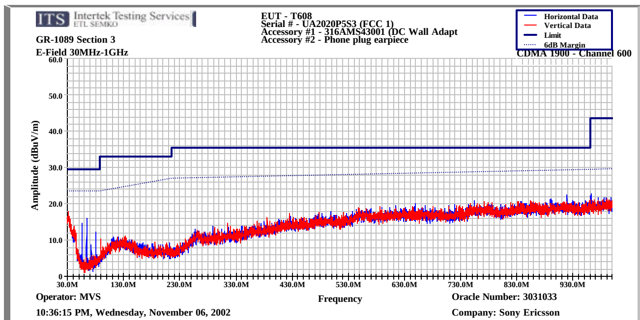
Figure 13-1 FCC §15.109, IC RSS-129, and IC RSS-133 Worst Case Receiver Spurious Emissions
