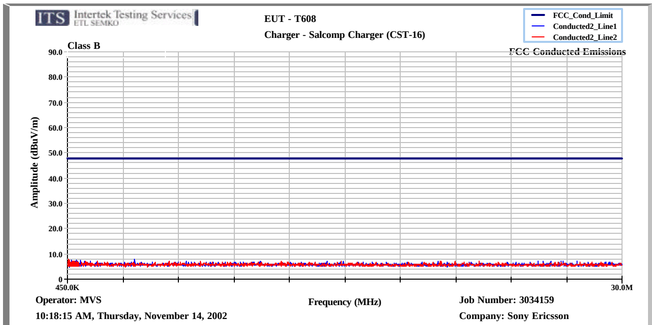
Figure 10-1: FCC §15.107 and §15.207 power line conducted emissions (peak) (CST-16)
