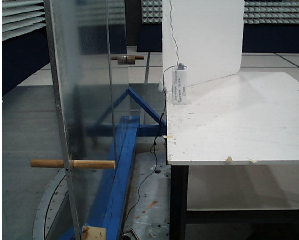
Figure 10-5: Configuration photograph, AC mains conducted emission, rear view
