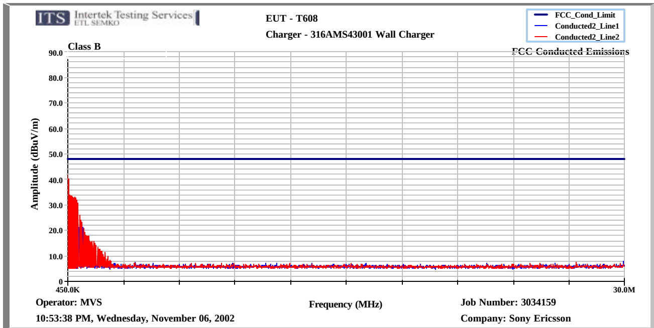
Figure 10-3: FCC §15.107 and §15.207 power line conducted emissions (peak) (CST-12)
