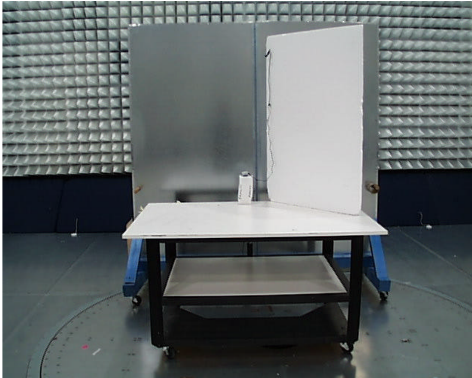
Figure 10-4: Configuration photograph, AC mains conducted emission, front view
