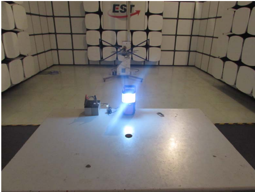
Car Charger Radiated Test (30-1000 MHz)
