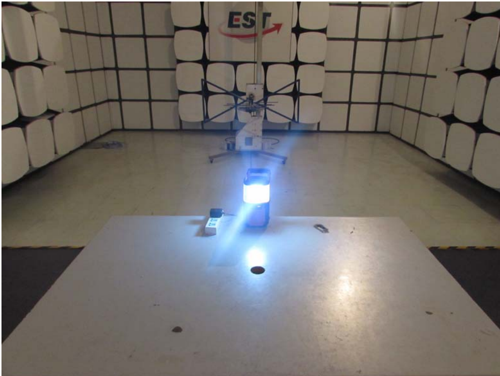
Adapter Radiated Test (30-1000 MHz)
