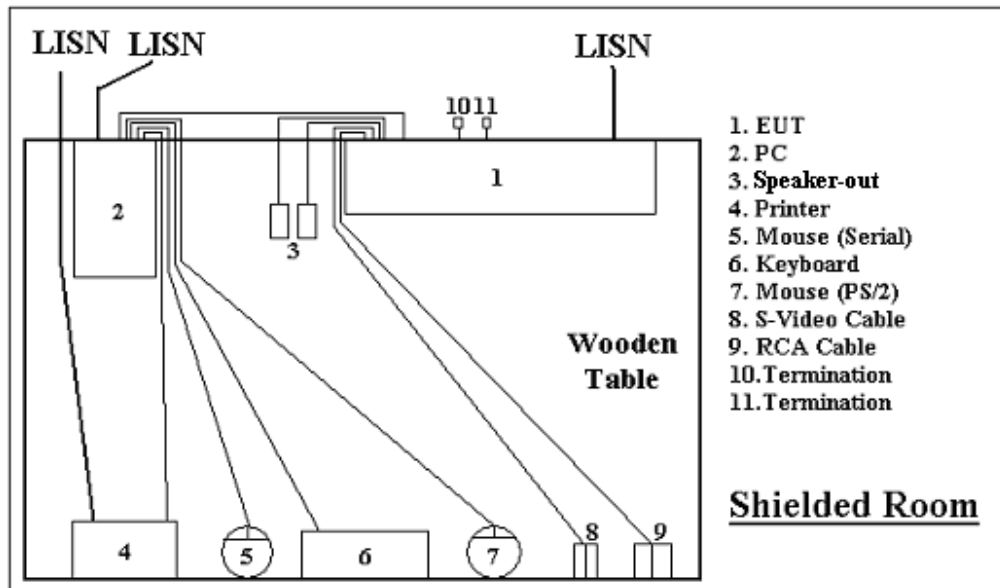
Conducted Emissions 150kHz - 30 MHz
