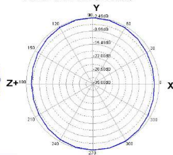
Passive Test E-Total (X-Y Plane)
