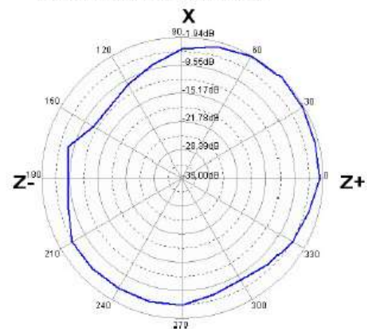
Passive Test E-Total (X-Z Plane)
