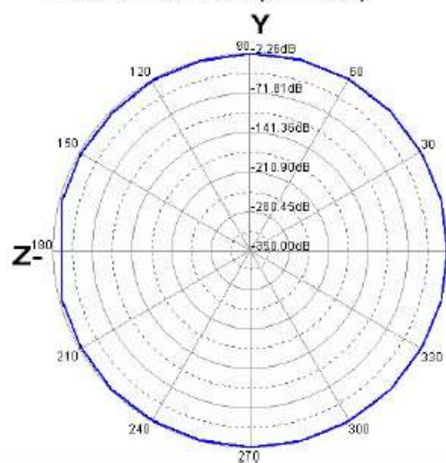
Passive Test E-Total (Y-Z Plane)
