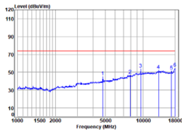
BLE_1M_TX_CH_00_Vertical-Peak
