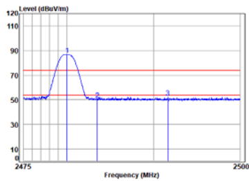
BLE_1M_TX_CH_39_Vertical
