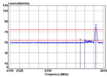
BLE_1M_TX_CH_00_Vertical
