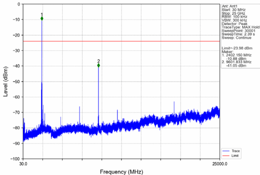
1M_LCH_2402MHz_Ant1_NTNV
