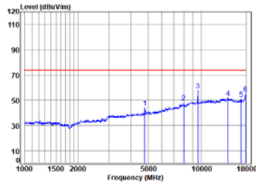
BLE_1M_TX_CH_00_Horizontal-Peak
