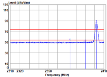
BLE_2M_TX_CH_00_Horizontal
