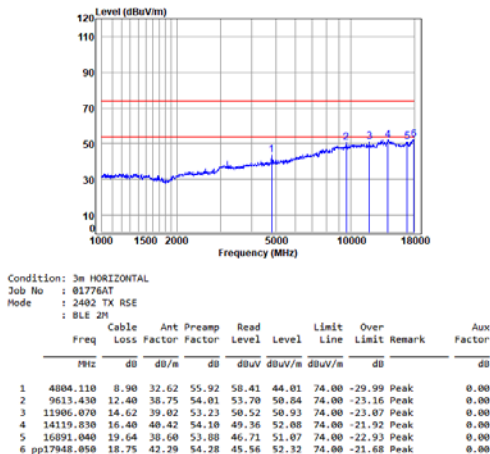
BLE_2M_TX_CH_00_Horizontal
