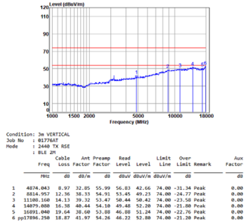
BLE_2M_TX_CH_19_Vertical
