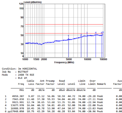
BLE_1M_TX_CH_39_Horizontal
