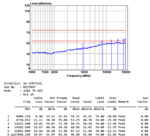
BLE_2M_TX_CH_00_Vertical
