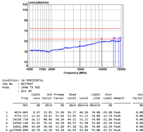
BLE_2M_TX_CH_19_Horizontal
