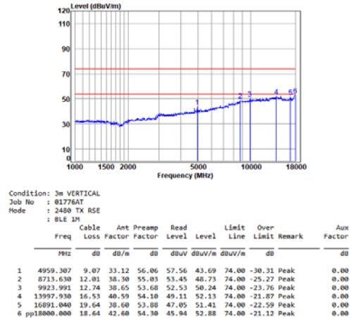
BLE_1M_TX_CH_39_Vertical
