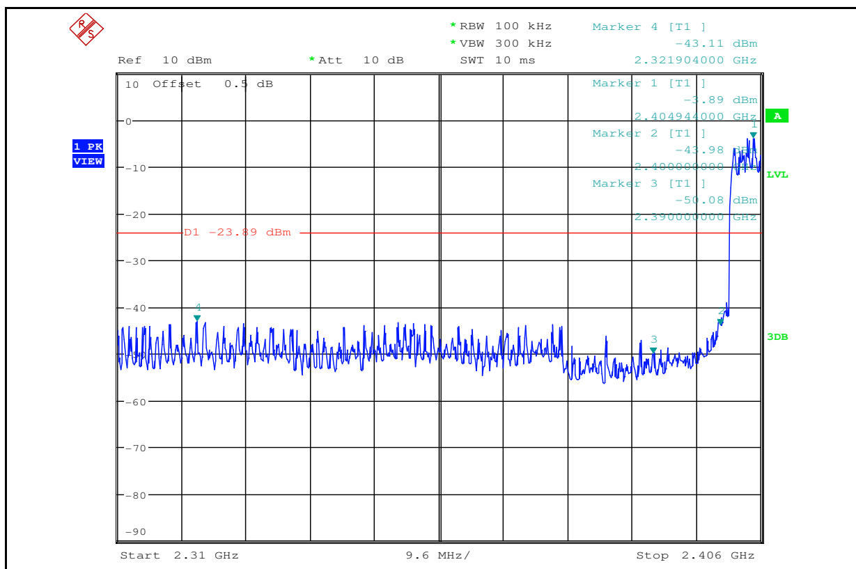
Band-edge for RF Conducted Emissions_3DH5_2402_Hopping Off
