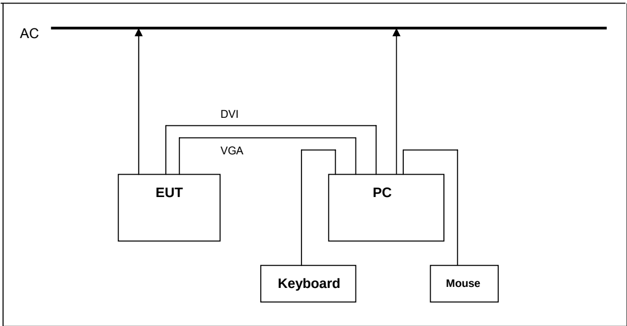
[ System Block Diagram of Test Configuration ]
