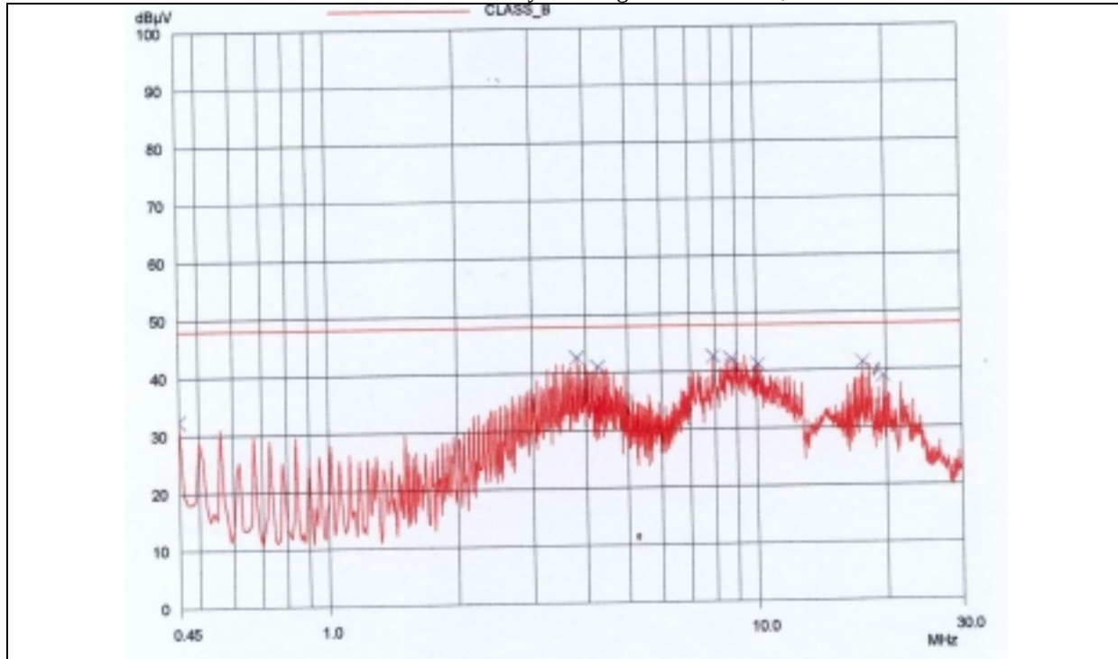
HOT LINE
