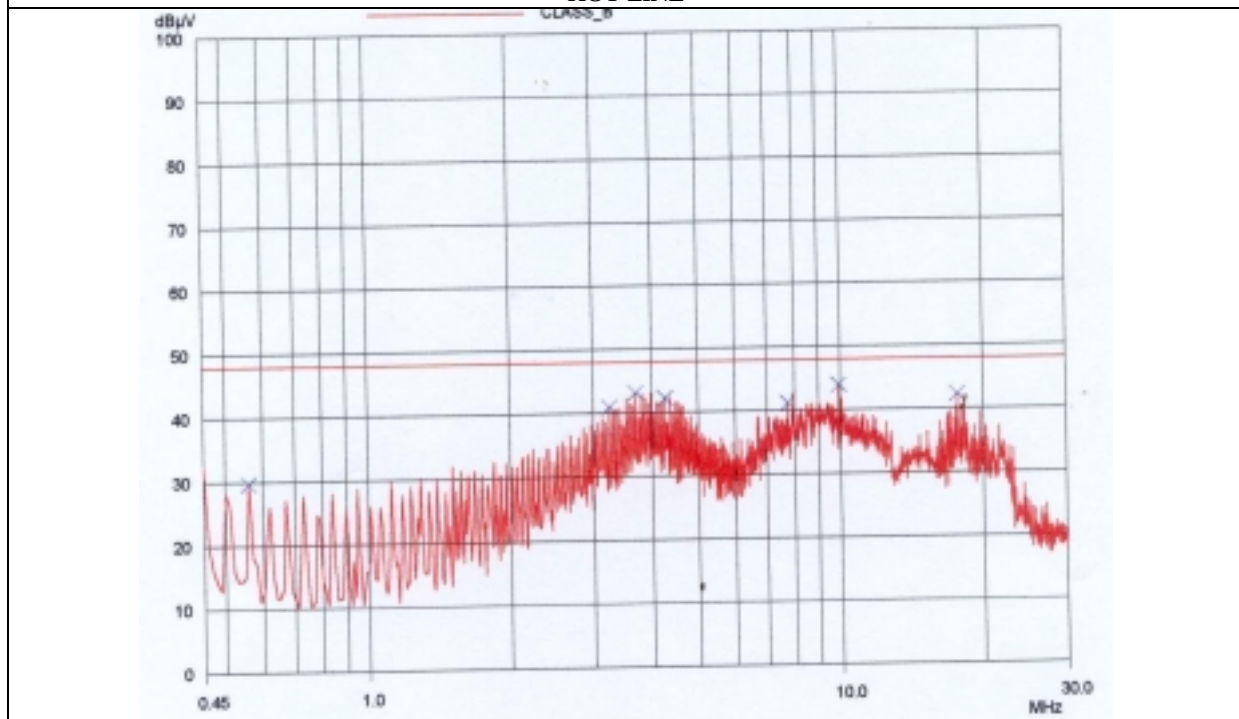
NEUTRAL LINE
