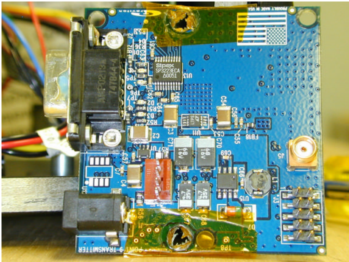
Radio Board Top
