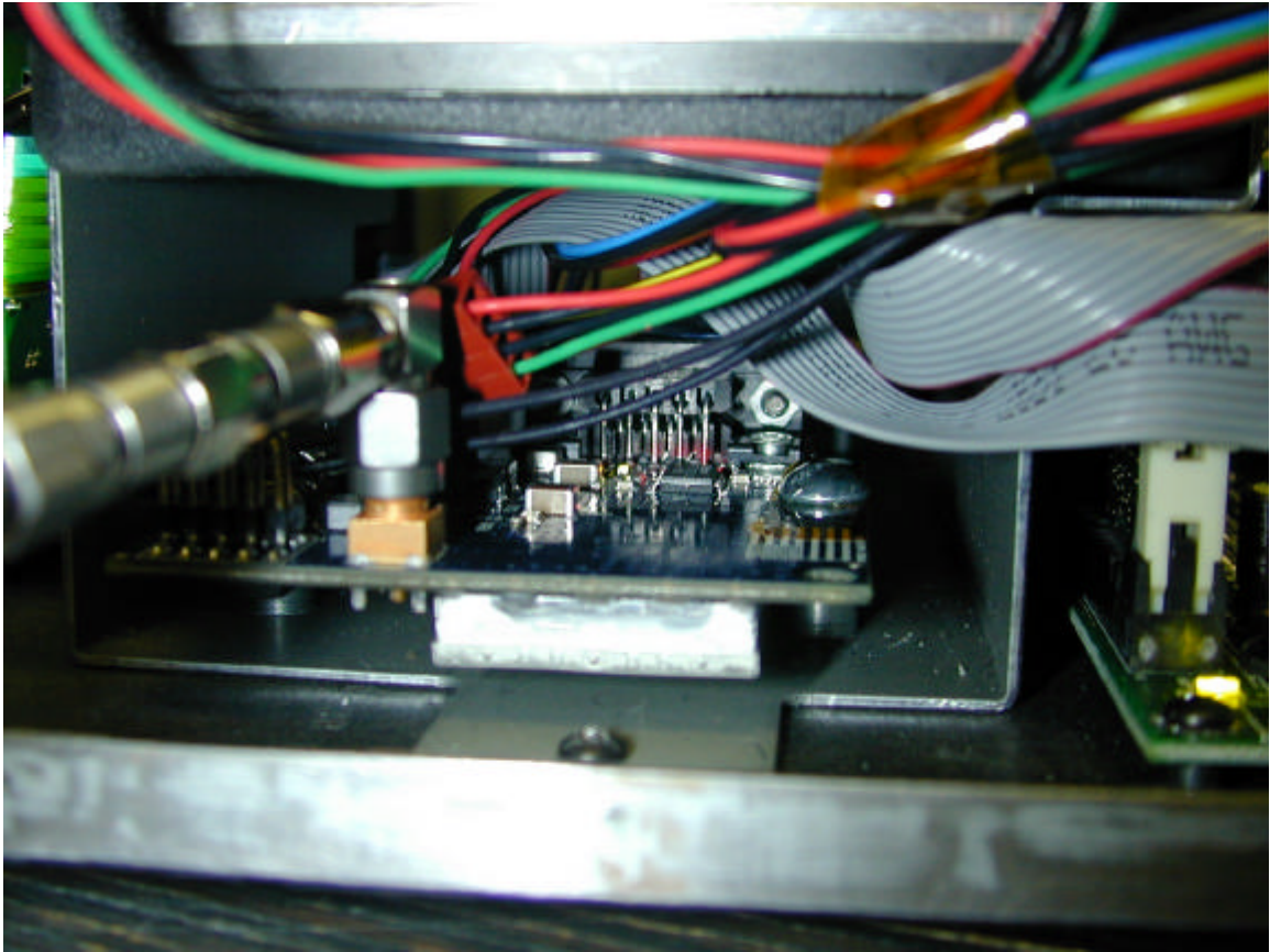
Radio Board mounted in MSG
