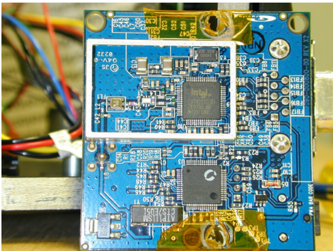
Radio Board –Bottom with Shield Removed
