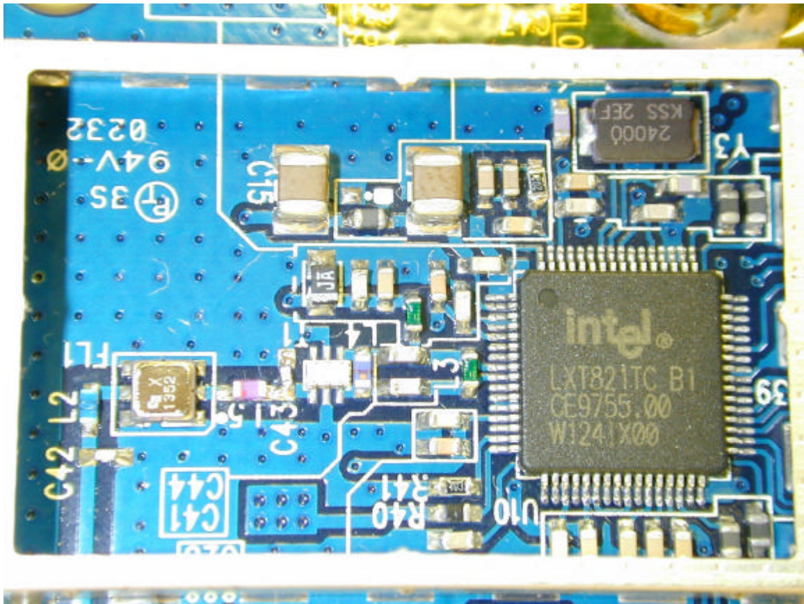
Radio Board – Close-up under shield
