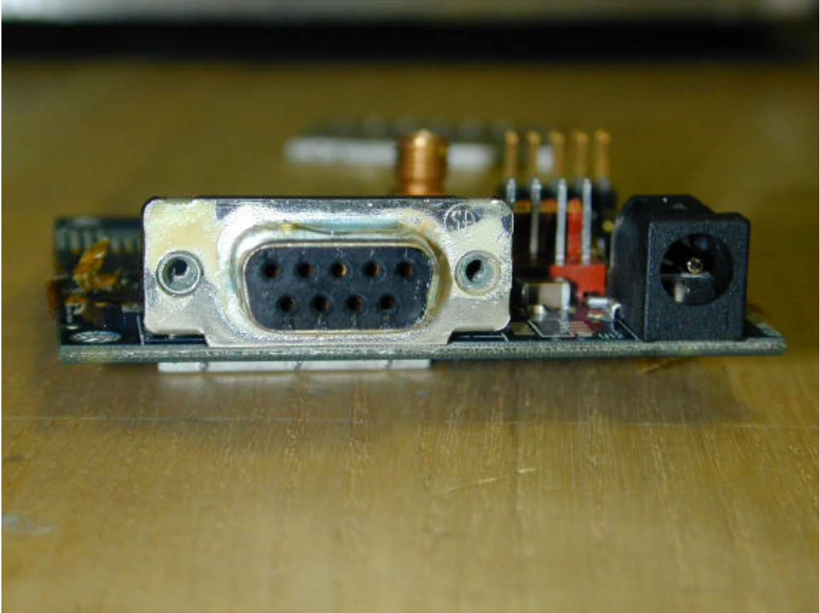
Radio Board – Data/Power Connector
