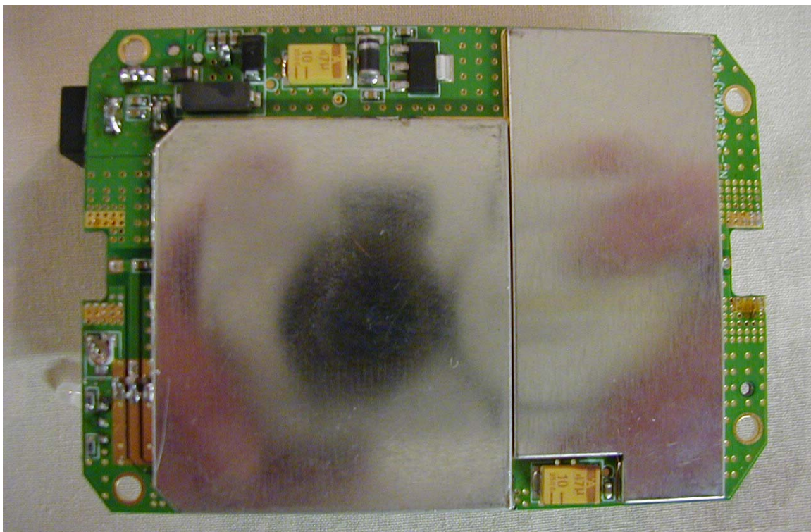
Component Side – With Shields
