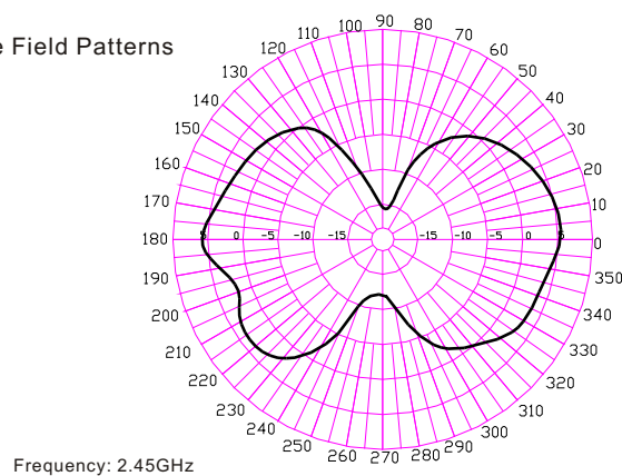
H-Plane Field Patterns
