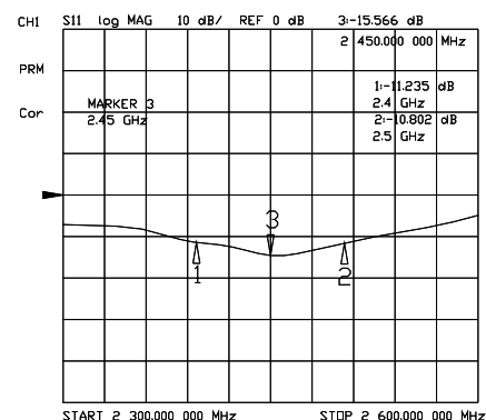
Return Loss
