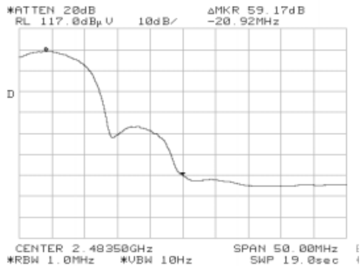
Average Bandedge
