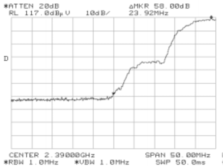
Peak Bandedge
