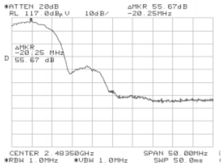
Peak Bandedge
