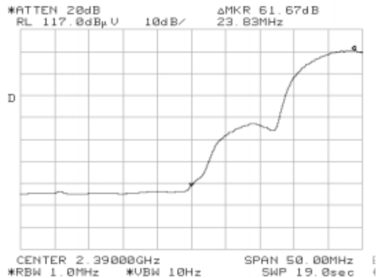
Average Bandedge
