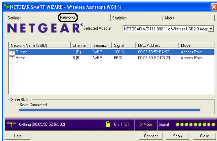
Figure 4-8: Networks page
