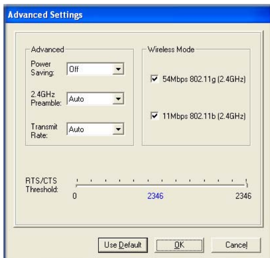
Figure 4-12: Advanced Settings
