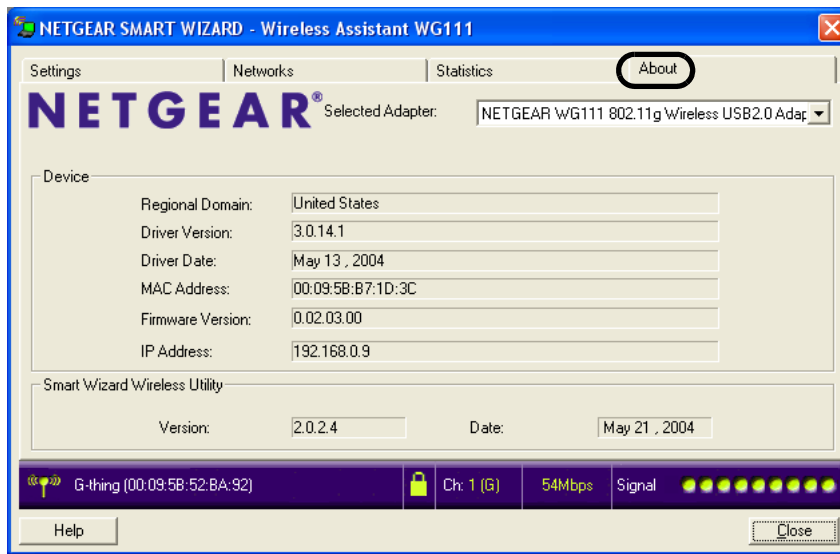
Figure 4-10: About page
