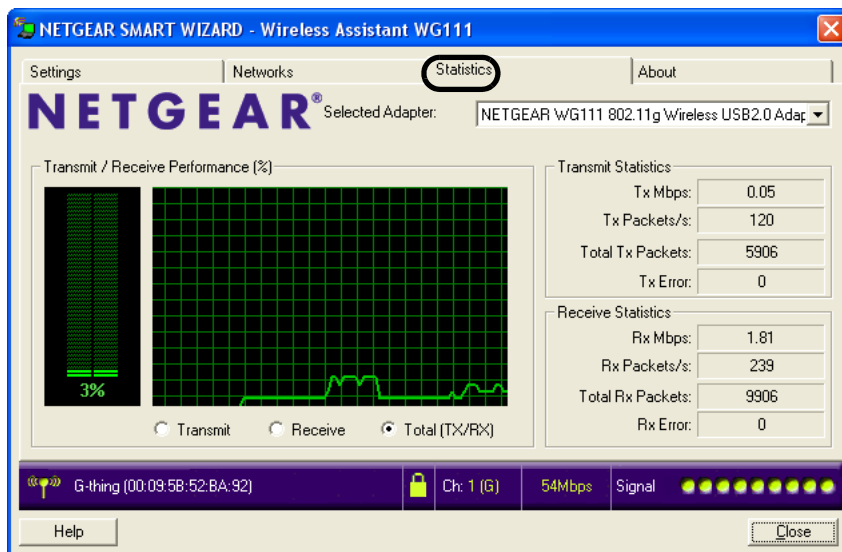
Figure 4-9: Statistics Page
