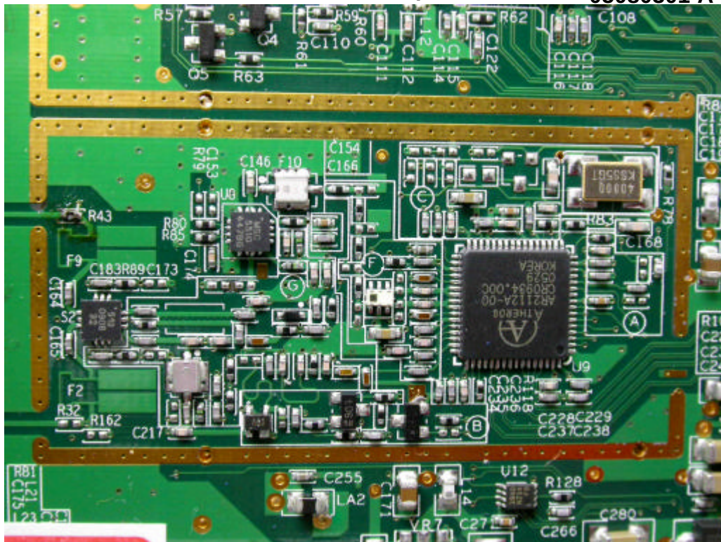
2.4GHz of RF part
