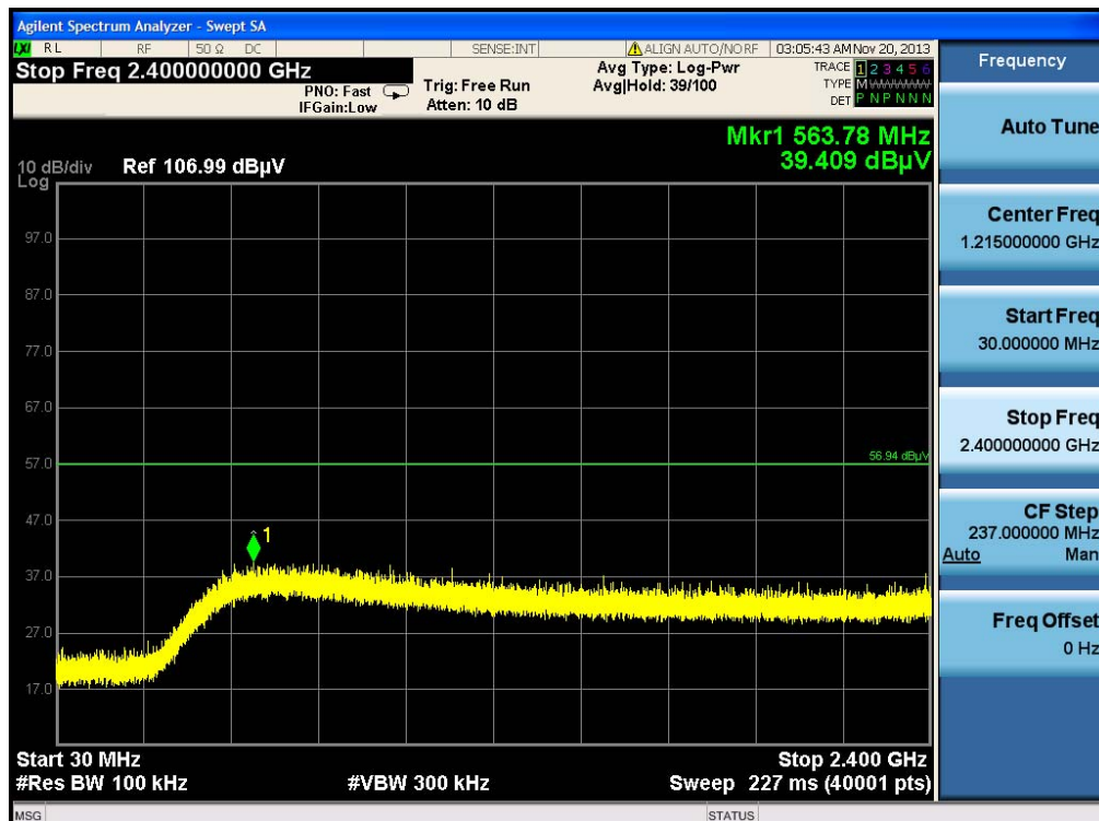
Plot on Configuration IEEE 802.11b / CH 11 / 30MHz~2400MHz (down 30dBc) / Ant. 1
