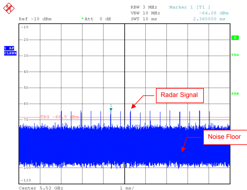
Radar Signal 2
